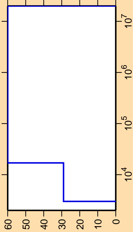
\Delta\sigma/\sigma vs. E for ^{93}\text{Sr}(n,\gamma)
