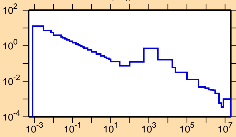
\sigma vs. E for ^{93}\text{Sr}(n,\gamma)
