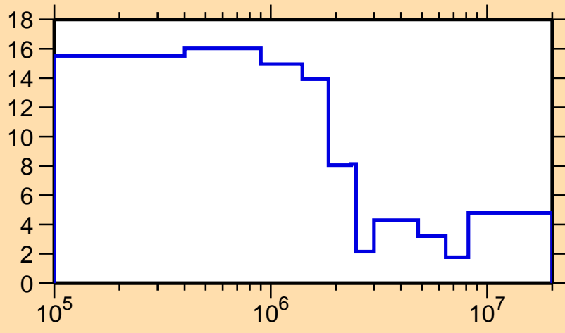
\Delta\sigma/\sigma vs. E for ^{93}\text{Sr}(n,\text{tot.})
