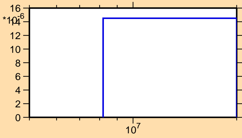
\sigma vs. E for ^{93}\text{Sr}(n,\alpha)
