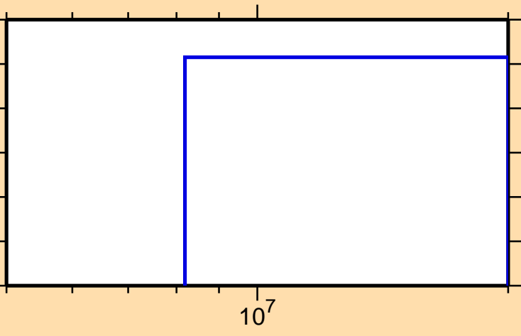
\sigma vs. E for ^{93}\text{Sr}(n,t)
