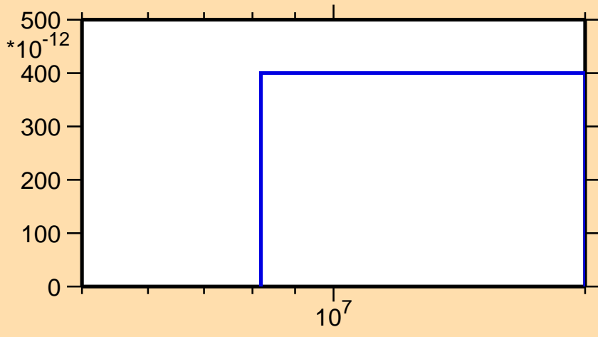
\sigma vs. E for ^{93}\text{Sr}(n,2n\alpha)
