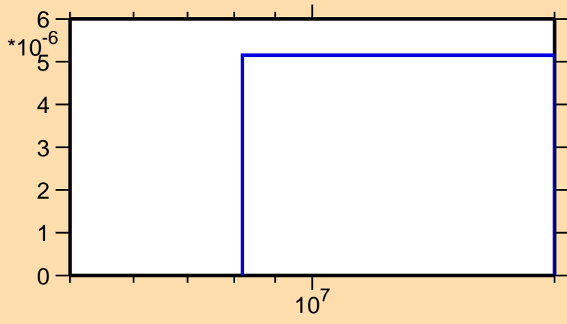
\sigma vs. E for ^{93}\text{Sr}(n,t)
