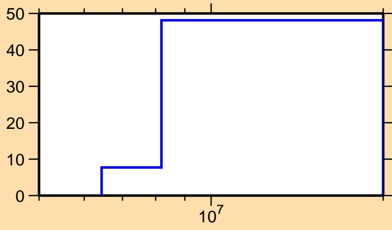
\Delta\sigma/\sigma vs. E for ^{93}\text{Sr}(n,p)
