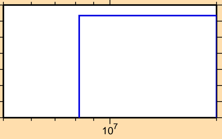
\sigma vs. E for ^{94}\text{Sr}(n,3n)
