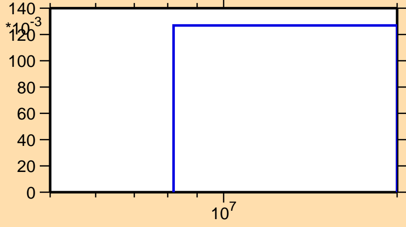
\sigma vs. E for ^{94}\text{Sr}(n,3n)
