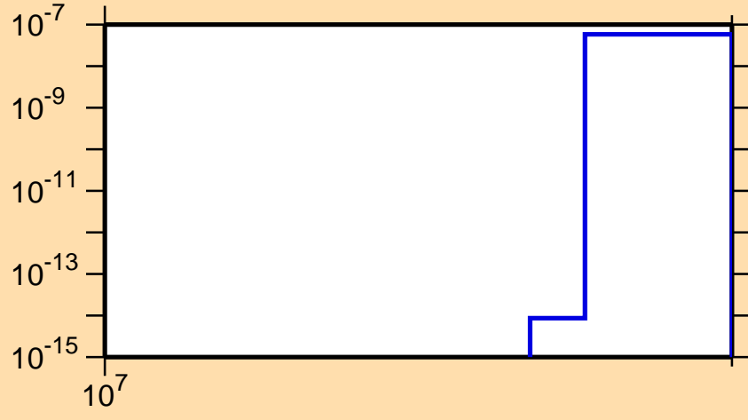
\sigma vs. E for ^{95}\text{Sr}(n,\text{nd})
