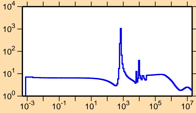
\sigma vs. E for ^{95}\text{Sr}(n,\text{el.})
