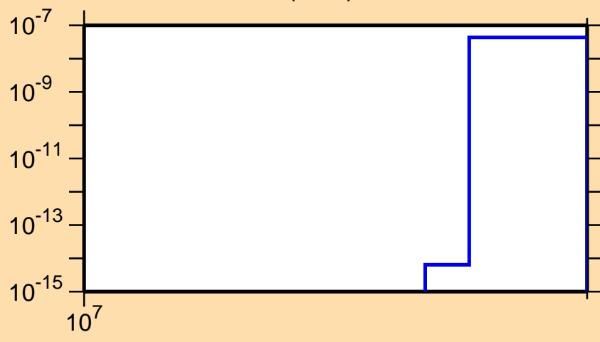
\sigma vs. E for ^{95}\text{Sr}(n,nt)
