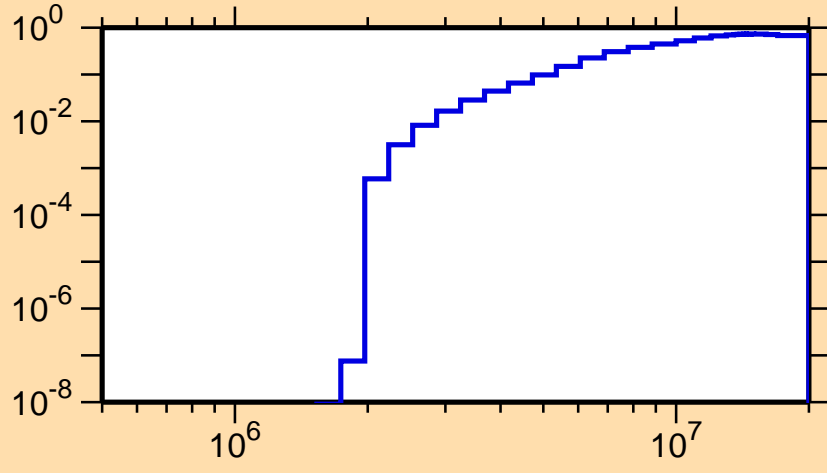
\sigma vs. E for ^{159}\text{Ta}(n,np)
