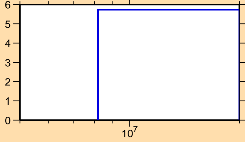
\Delta\sigma/\sigma vs. E for ^{159}\text{Ta}(n,\text{el.})
