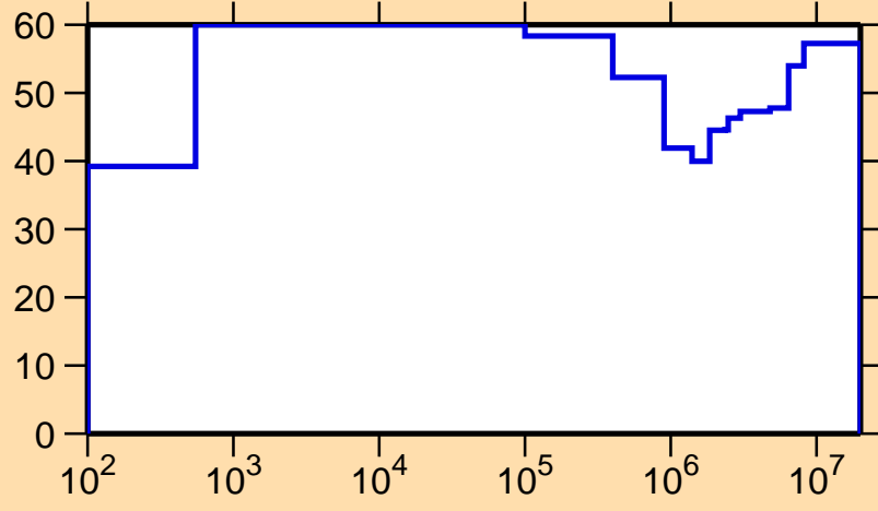
\Delta\sigma/\sigma vs. E for ^{159}\text{Ta}(n,p)
