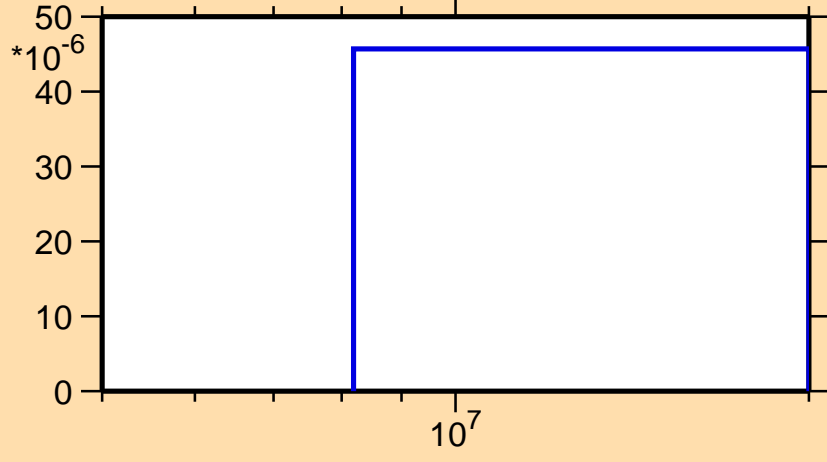
\sigma vs. E for ^{159}\text{Ta}(n,2n\alpha)
