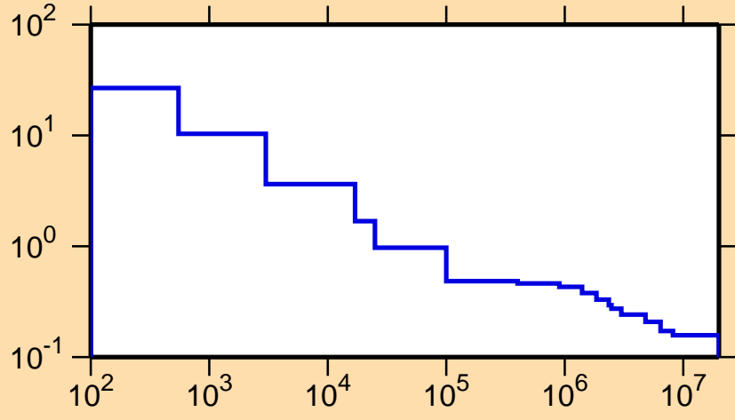
\sigma vs. E for ^{159}\text{Ta}(n,p\alpha)
