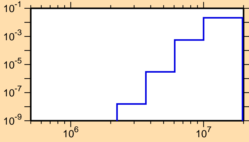
\sigma vs. E for ^{160}\text{Ta}(n,d)
