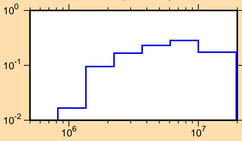
\sigma vs. E for ^{160}\text{Ta}(n,n\text{cont.})
