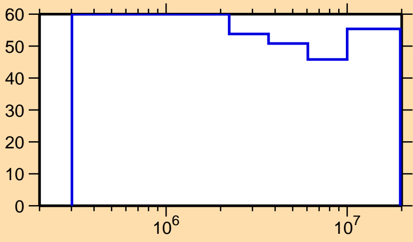
\Delta\sigma/\sigma vs. E for ^{160}\text{Ta}(n,n_1)
