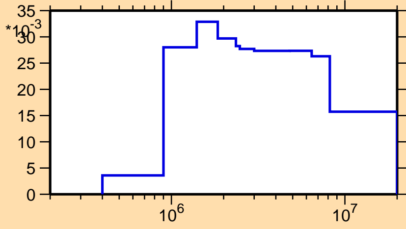
\sigma vs. E for ^{160}\text{Ta}(n,n_4)
