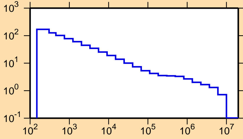
\sigma vs. E for ^{160}\text{Ta}(n,p)
