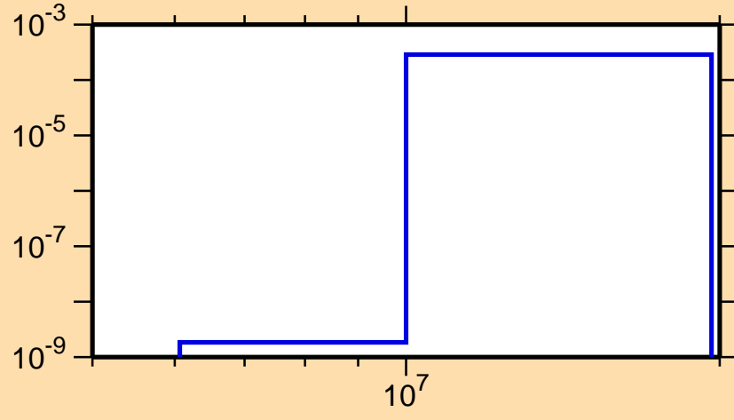
\sigma vs. E for ^{160}\text{Ta}(n,pd)
