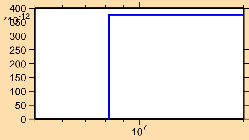
\sigma vs. E for ^{160}\text{Ta}(n,nt)
