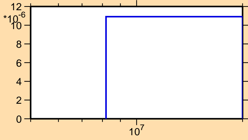
\sigma vs. E for ^{160}\text{Ta}(n,\text{pt})
