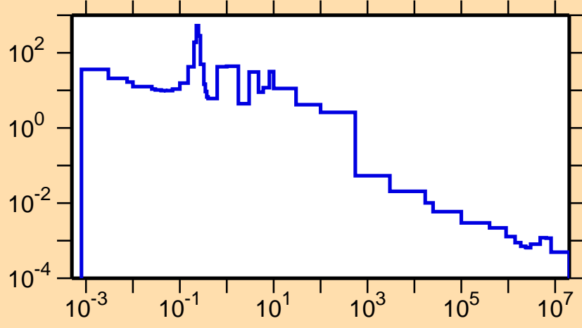
\sigma vs. E for ^{160}\text{Ta}(n,\gamma)
