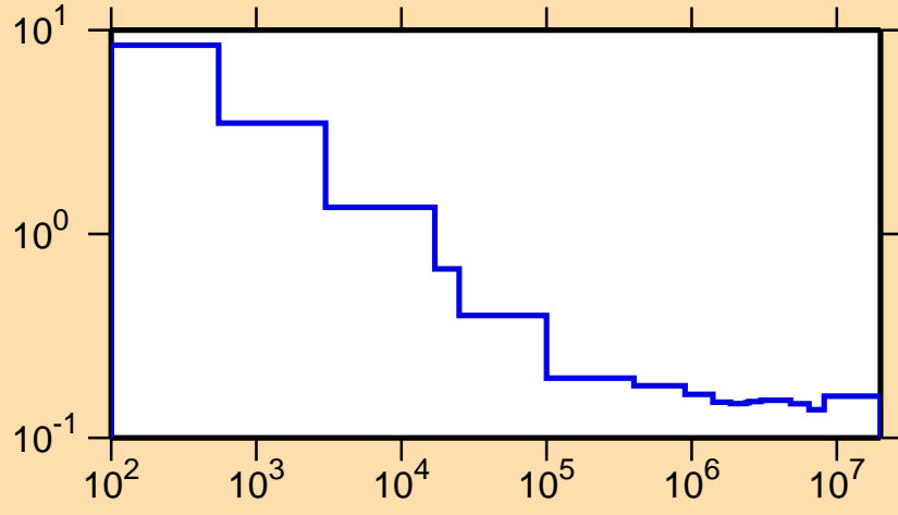
\sigma vs. E for ^{160}\text{Ta}(n,p\alpha)
