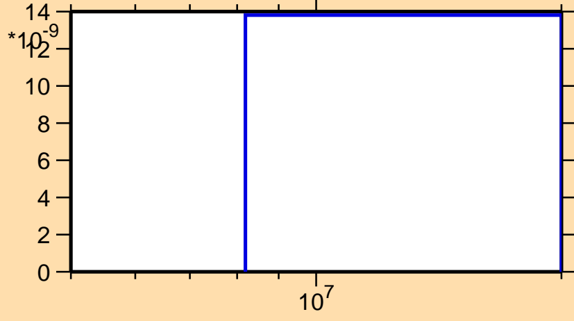
\sigma vs. E for ^{160}\text{Ta} (mt 34)
