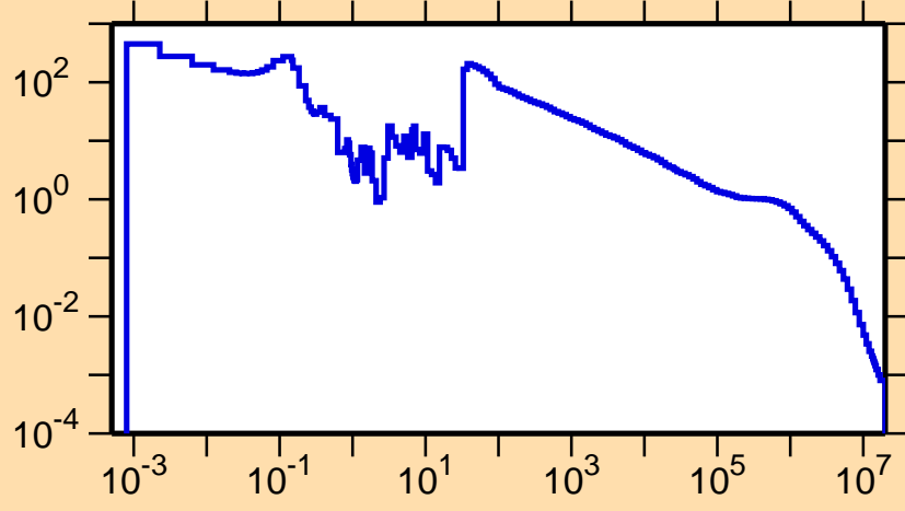
\sigma vs. E for ^{161}\text{Ta}(n,\gamma)
