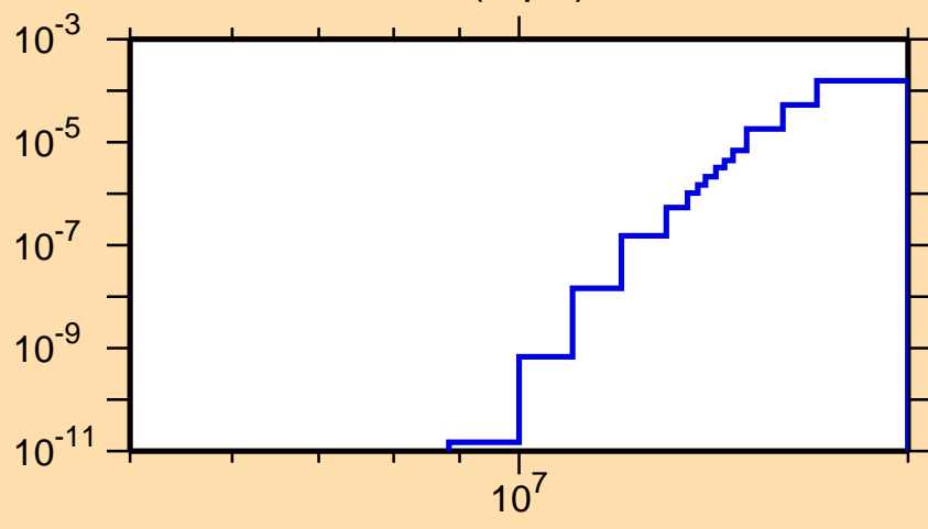
\sigma vs. E for ^{162}\text{Ta}(n,\text{pd})
