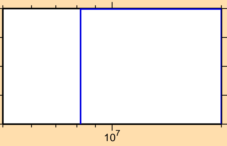
\sigma vs. E for ^{162}\text{Ta}(n,2np)
