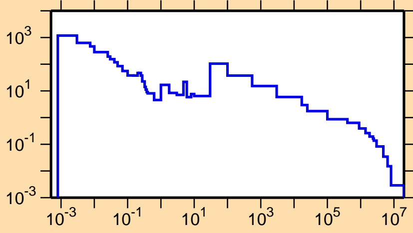
\sigma vs. E for ^{162}\text{Ta}(n,\gamma)
