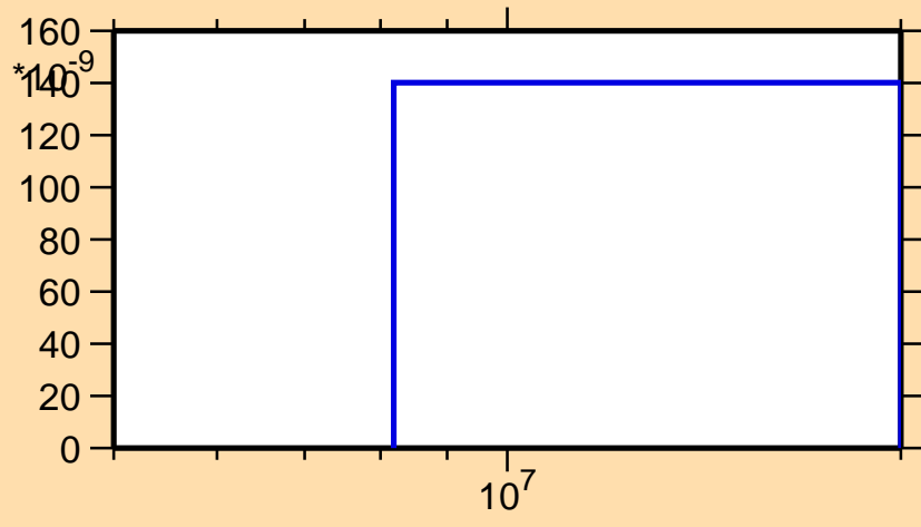
\sigma vs. E for ^{162}\text{Ta}(n,\text{pt})
