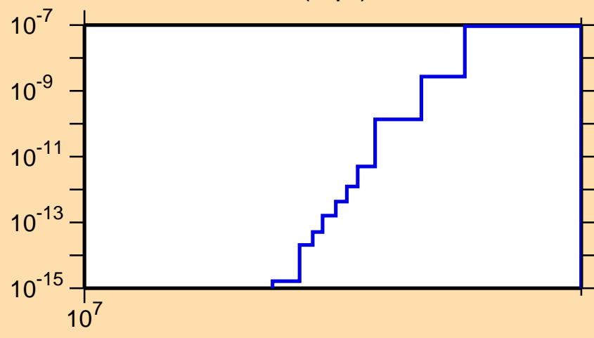
\sigma vs. E for ^{163}\text{Ta}(n,\text{pt})
