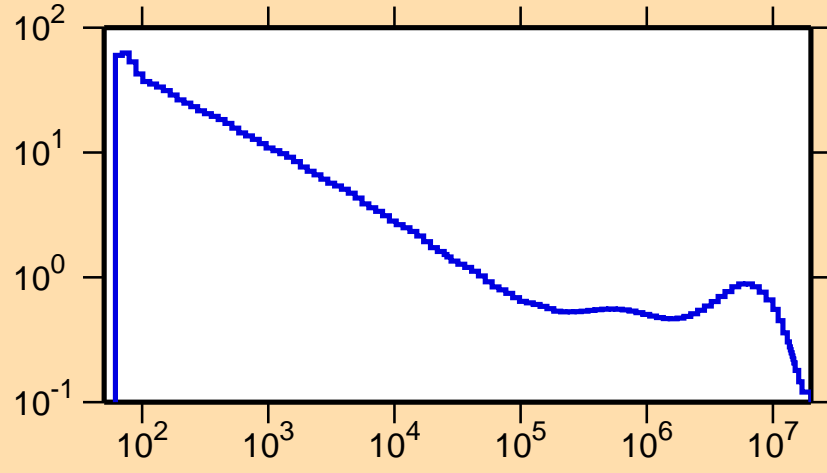
\sigma vs. E for ^{163}\text{Ta}(n,p)
