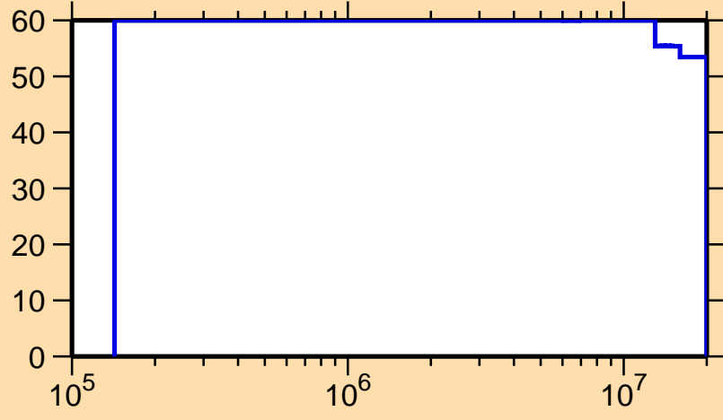
\Delta\sigma/\sigma vs. E for ^{163}\text{Ta}(n,n\text{cont.})
