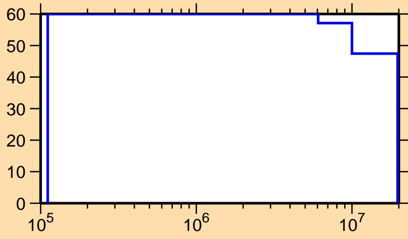
\Delta\sigma/\sigma vs. E for ^{163}\text{Ta}(n,n_1)
