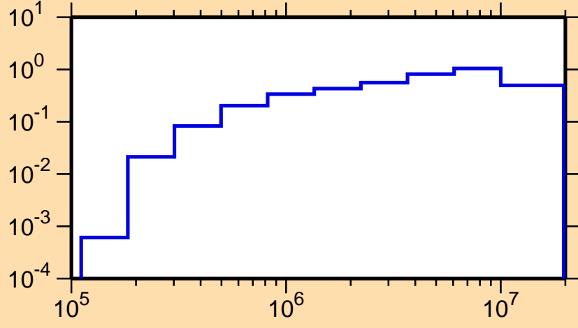
\sigma vs. E for ^{163}\text{Ta}(n,\text{inel.})
