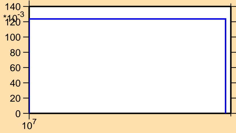
\sigma vs. E for ^{163}\text{Ta}(n,2n)
