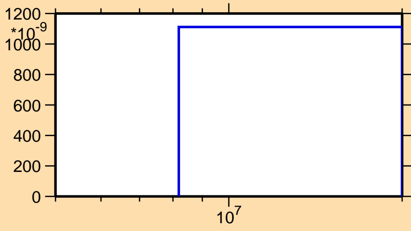
\sigma vs. E for ^{163}\text{Ta}(n,pd)
