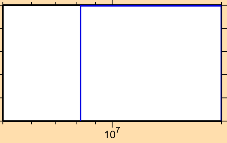
\sigma vs. E for ^{163}\text{Ta}(n,2n)
