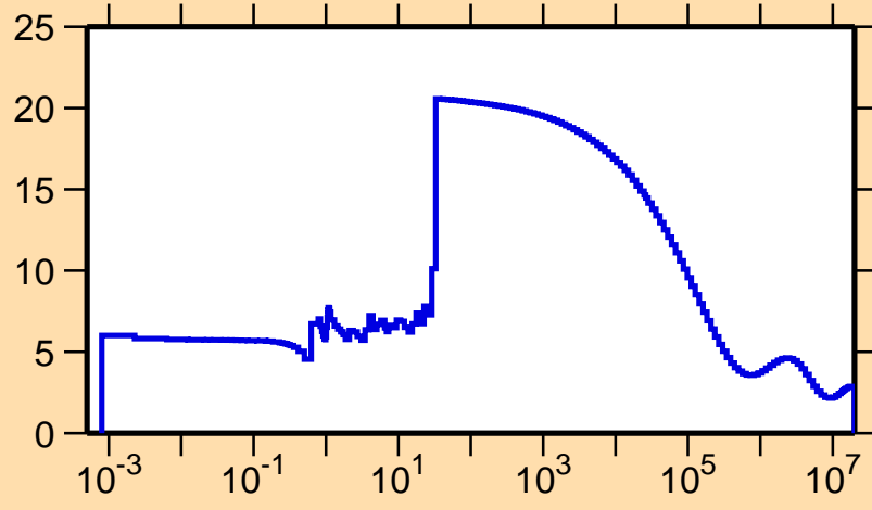
\sigma vs. E for ^{164}\text{Ta}(n,\text{el.})
