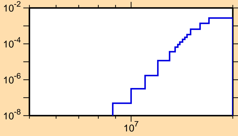
\sigma vs. E for ^{164}\text{Ta}(n,2n\alpha)
