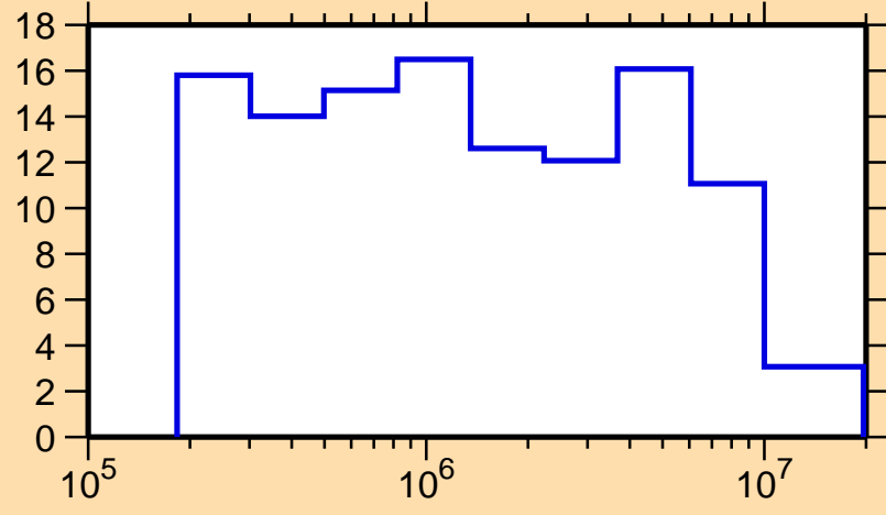
\Delta\sigma/\sigma vs. E for ^{164}\text{Ta}(n,tot.)
