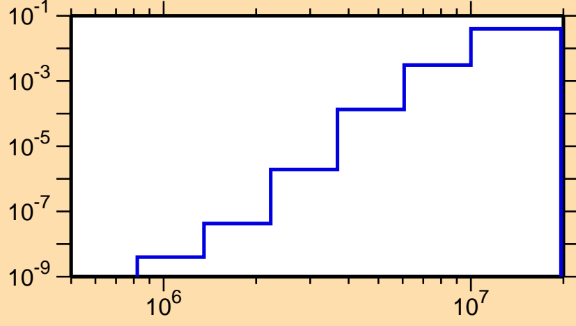
\sigma vs. E for ^{164}\text{Ta}(n,n\alpha)
