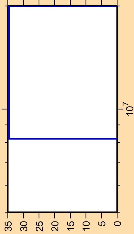
\Delta\sigma/\sigma vs. E for ^{164}\text{Ta}(n,3n\alpha)
