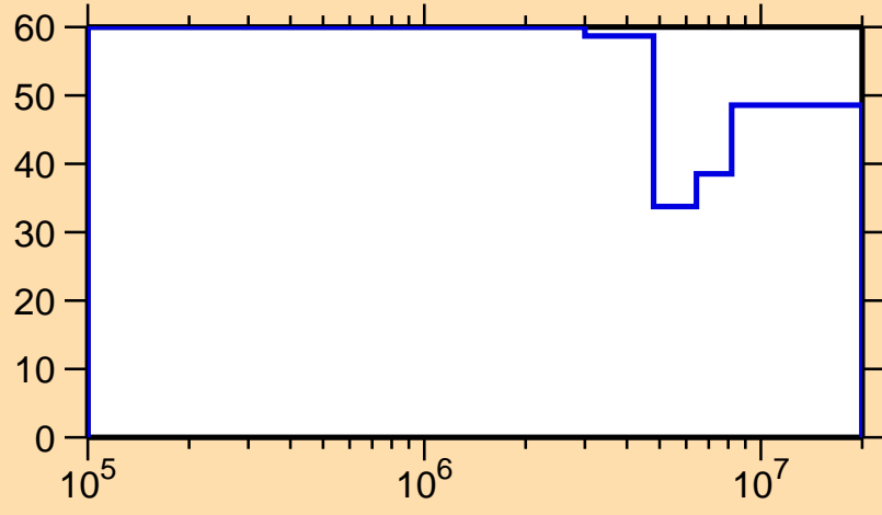
\Delta\sigma/\sigma vs. E for ^{164}\text{Ta}(n,n\text{cont.})
