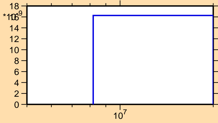
\sigma vs. E for ^{164}\text{Ta}(n,3n\alpha)
