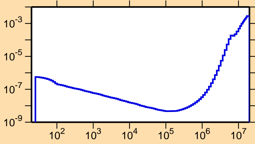
\sigma vs. E for ^{165}\text{Ta}(n,p\alpha)
