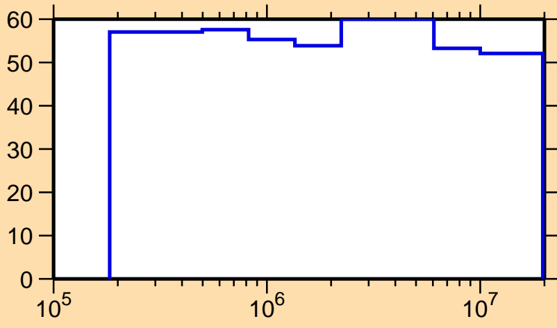
\Delta\sigma/\sigma vs. E for ^{165}\text{Ta}(n,n\text{cont.})
