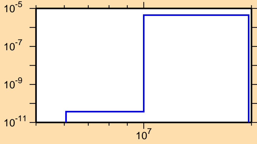
\sigma vs. E for ^{165}\text{Ta}(n,\text{He3})
