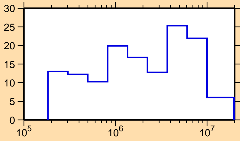
\Delta\sigma/\sigma vs. E for ^{165}\text{Ta}(n,el.)
