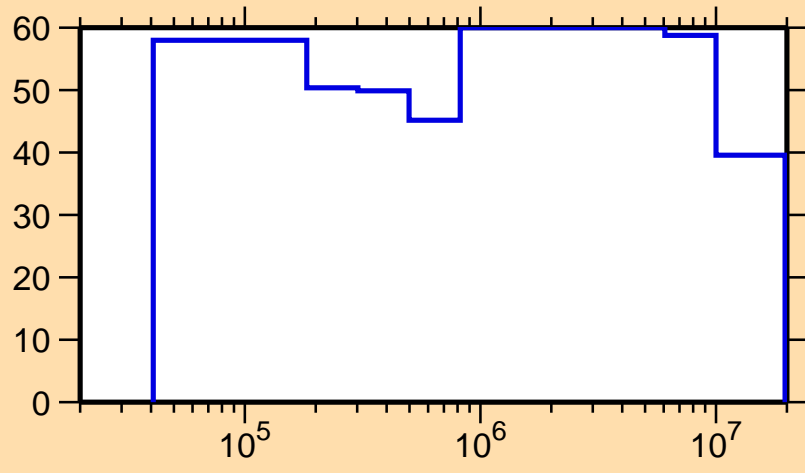
\Delta\sigma/\sigma vs. E for ^{165}\text{Ta}(n,n_1)
