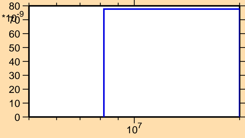
\sigma vs. E for ^{165}\text{Ta}(n,pd)
