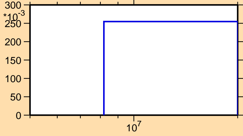
\sigma vs. E for ^{165}\text{Ta}(n,2n)
