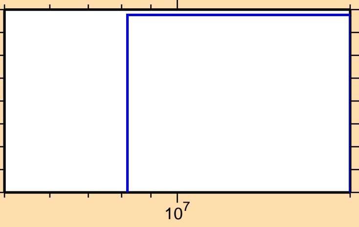
\sigma vs. E for ^{165}\text{Ta}(n,pd)
