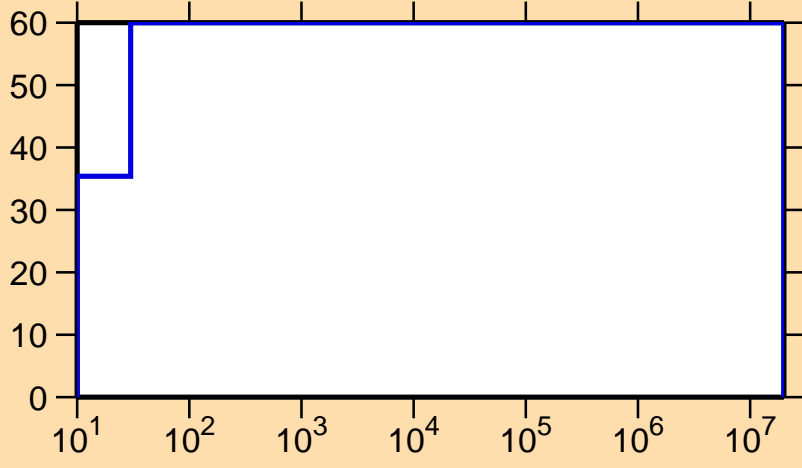
\Delta\sigma/\sigma vs. E for ^{165}\text{Ta}(n,p)
