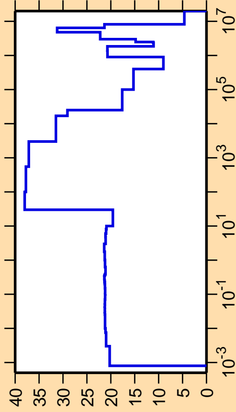
\Delta\sigma/\sigma vs. E for ^{165}\text{Ta}(n,\text{el.})
