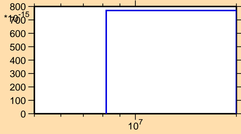
\sigma vs. E for ^{165}\text{Ta} (mt 34)
