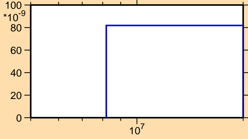
\sigma vs. E for ^{165}\text{Ta}(n,\text{nd})
