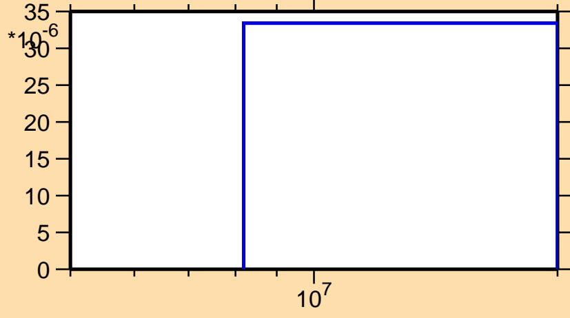
\sigma vs. E for ^{165}\text{Ta}(n,2np)
