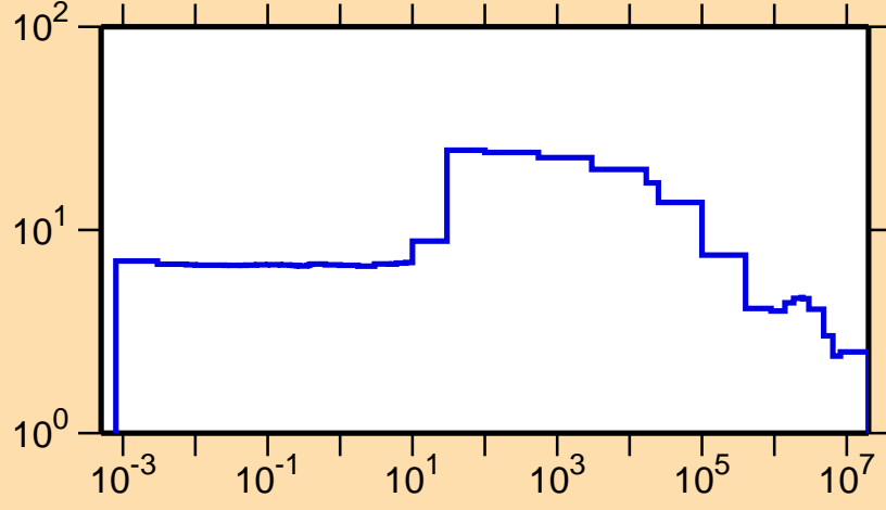
\sigma vs. E for ^{165}\text{Ta}(n,\text{el.})
