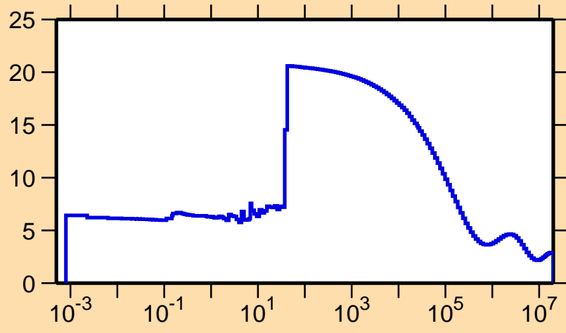
\sigma vs. E for ^{166}\text{Ta}(n,\text{el.})
