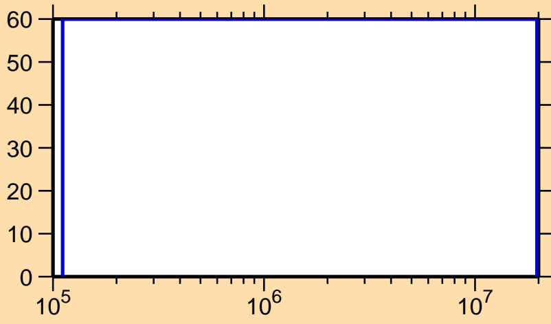
\Delta\sigma/\sigma vs. E for ^{166}\text{Ta}(n,n_1)
