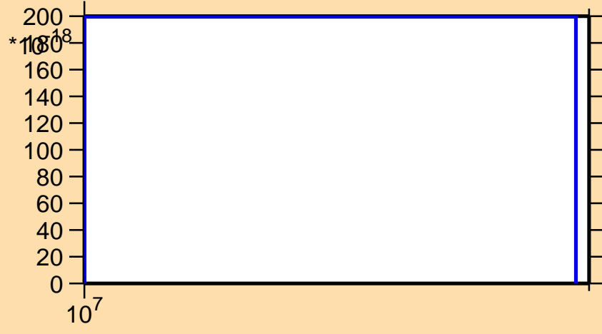
\sigma vs. E for ^{166}\text{Ta}(n,3n\alpha)
