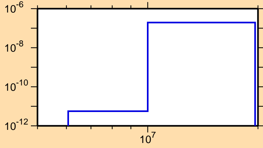
\sigma vs. E for ^{166}\text{Ta}(\text{mt117})
