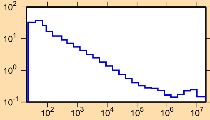
\sigma vs. E for ^{166}\text{Ta}(n,p)
