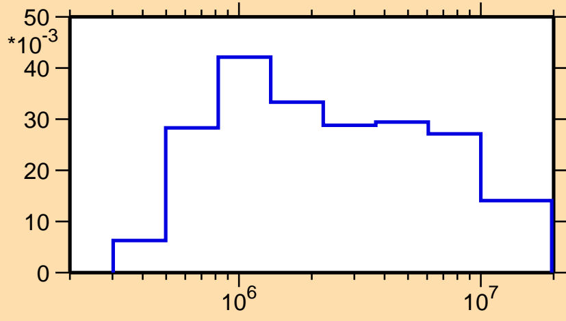
\sigma vs. E for ^{166}\text{Ta}(n,n_3)
