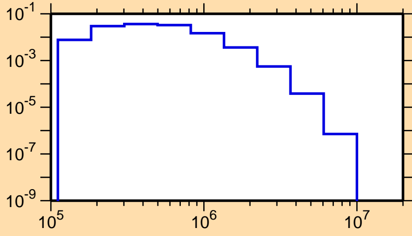
\sigma vs. E for ^{166}\text{Ta}(n,n_1)
