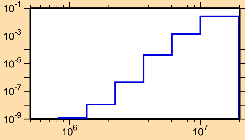
\sigma vs. E for ^{166}\text{Ta}(n,n\alpha)
