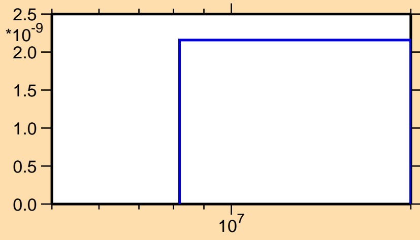
\sigma vs. E for ^{166}\text{Ta}(n,\text{pt})
