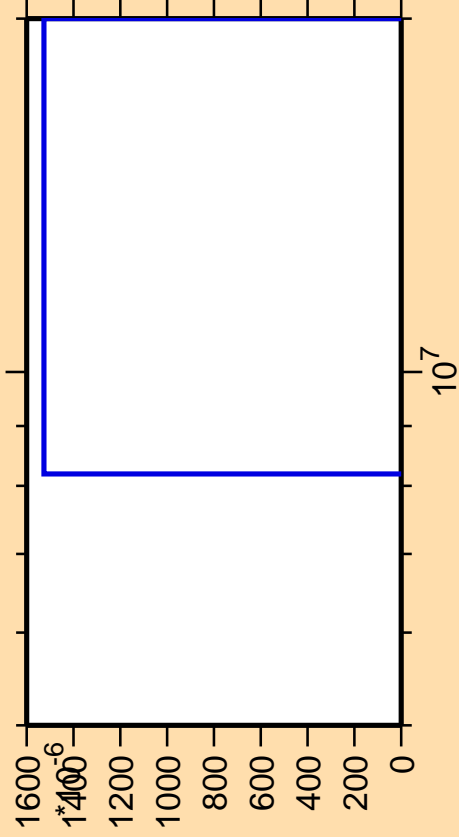
\Delta\sigma/\sigma vs. E for ^{166}\text{Ta}(n,3n\alpha)
