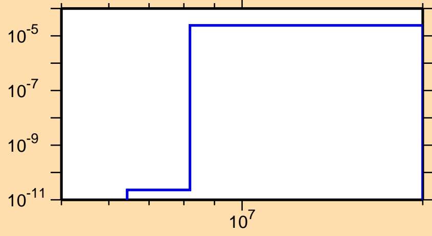
\sigma vs. E for ^{166}\text{Ta} (mt 45)
