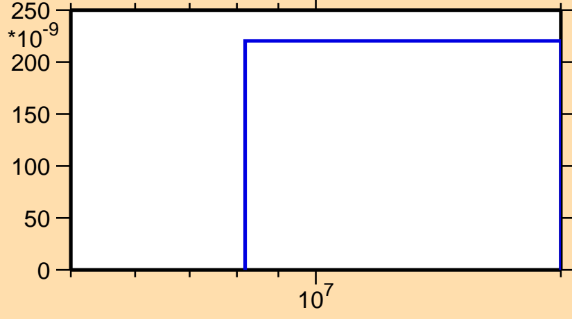
\sigma vs. E for ^{166}\text{Ta}(n,3n)
