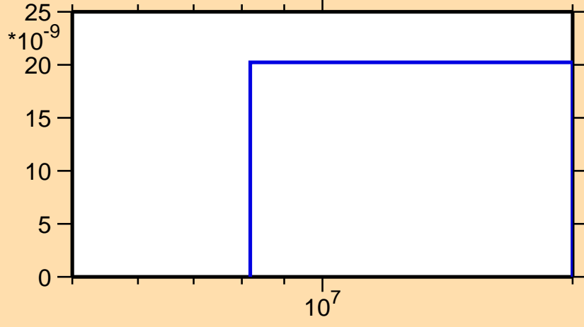
\sigma vs. E for ^{166}\text{Ta}(n,pd)
