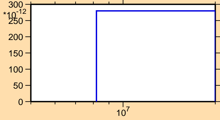
\sigma vs. E for ^{166}\text{Ta}(n,nt)
