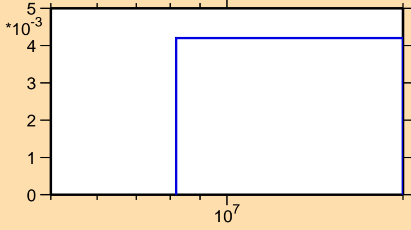
\sigma vs. E for ^{166}\text{Ta}(n,2np)
