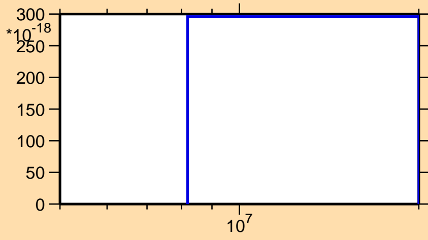
\sigma vs. E for ^{166}\text{Ta}(n,3n\alpha)
