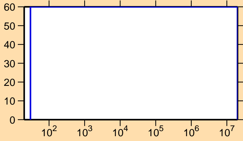
\Delta\sigma/\sigma vs. E for ^{166}\text{Ta}(n,\gamma)
