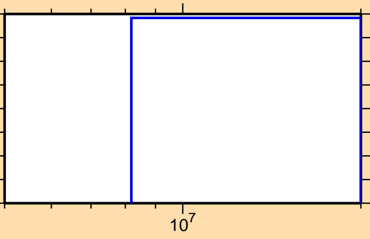
\sigma vs. E for ^{166}\text{Ta}(n,2n\alpha)
