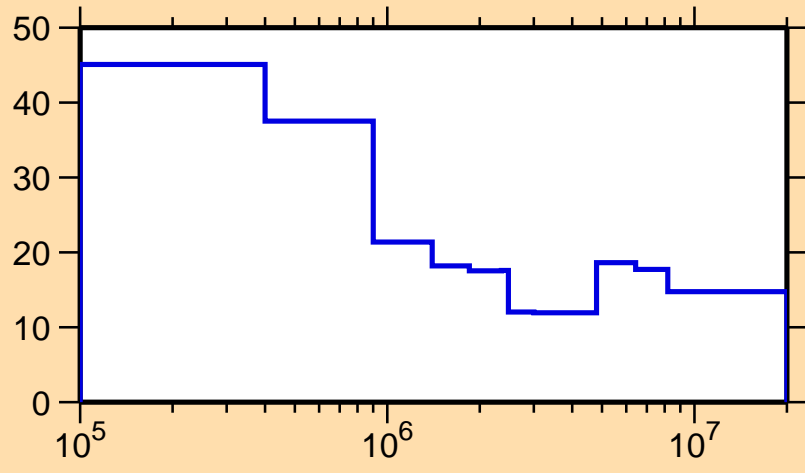
\Delta\sigma/\sigma vs. E for ^{166}\text{Ta}(n,\text{nonel.})
