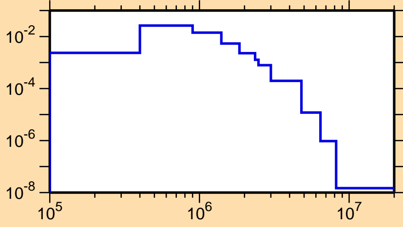
\sigma vs. E for ^{166}\text{Ta}(n,n_2)
