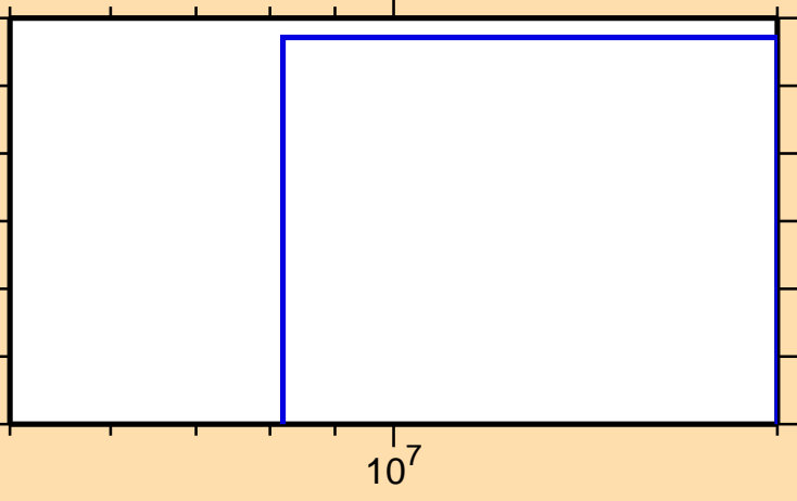
\sigma vs. E for ^{166}\text{Ta}(n,\text{nd})
