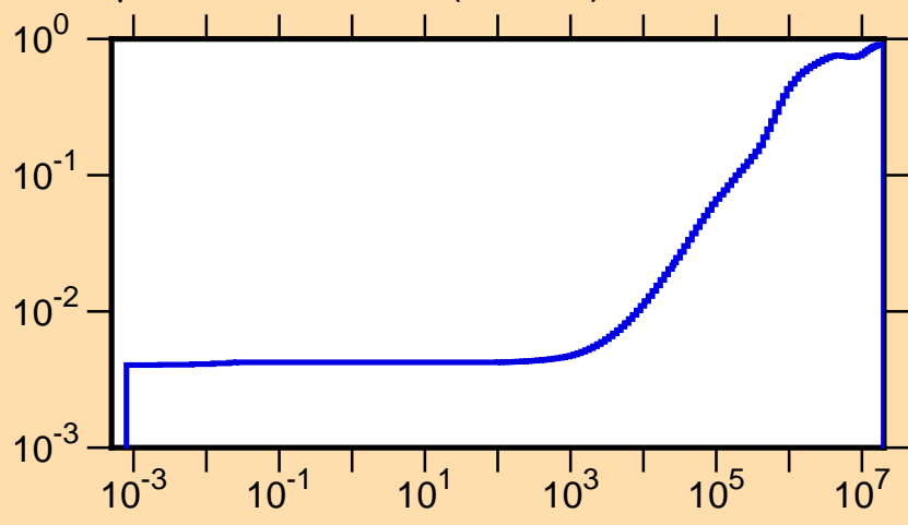
\mu vs. E for ^{167}\text{Ta}(\text{mt251})
