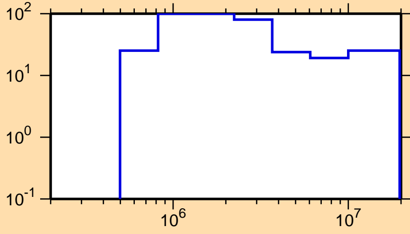
\Delta\sigma/\sigma vs. E for ^{167}\text{Ta}(n,n\text{cont.})
