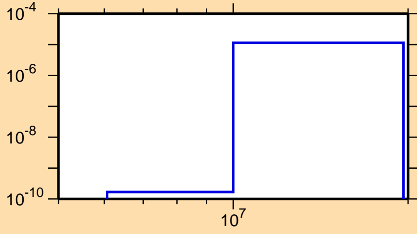
\sigma vs. E for ^{167}\text{Ta} (mt 45)
