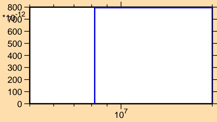
\sigma vs. E for ^{167}\text{Ta}(n,nt)
