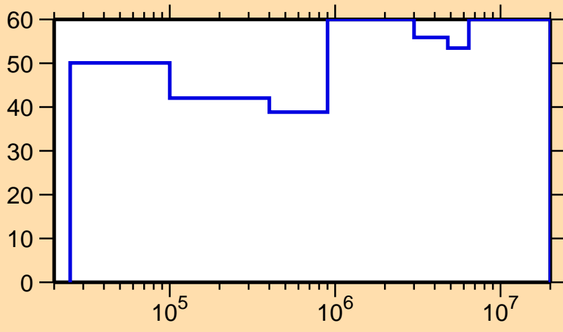
\Delta\sigma/\sigma vs. E for ^{167}\text{Ta}(n,n_1)
