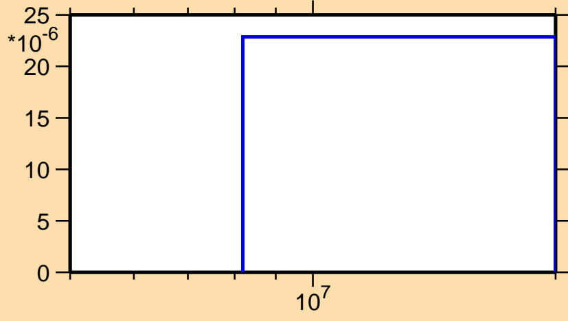
\sigma vs. E for ^{167}\text{Ta}(n,2np)
