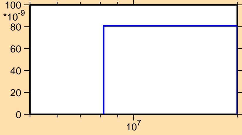
\sigma vs. E for ^{167}\text{Ta}(n,\text{nd})
