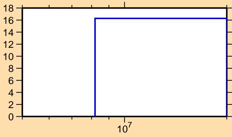
\Delta\sigma/\sigma vs. E for ^{167}\text{Ta}(n,\text{inel.})
