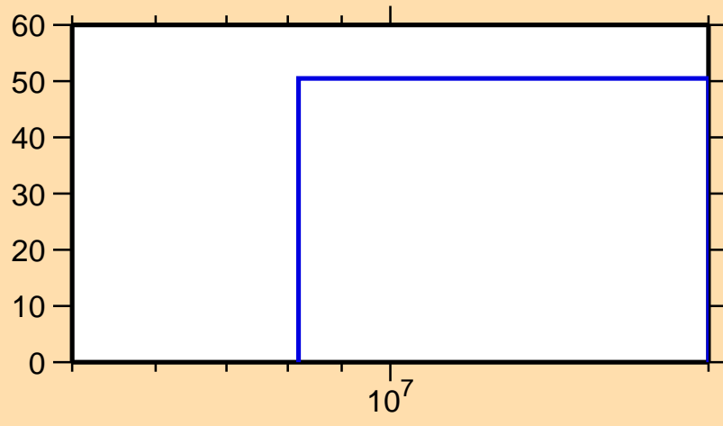
\Delta\sigma/\sigma vs. E for ^{167}\text{Ta}(n,2n)
