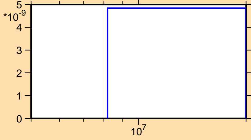
\sigma vs. E for ^{167}\text{Ta}(n,pd)
