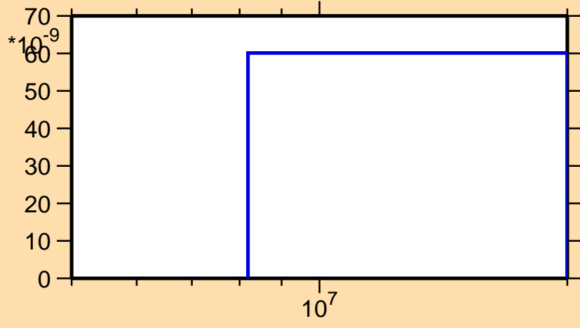
\sigma vs. E for ^{167}\text{Ta}(\text{mt117})
