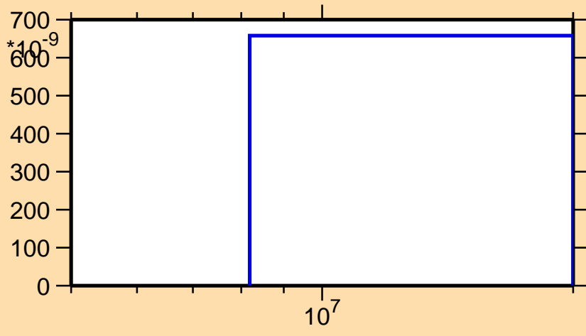
\sigma vs. E for ^{167}\text{Ta}(n,3n)
