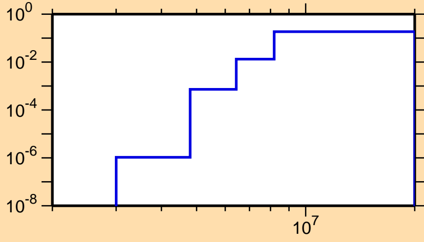
\sigma vs. E for ^{167}\text{Ta}(n,np)
