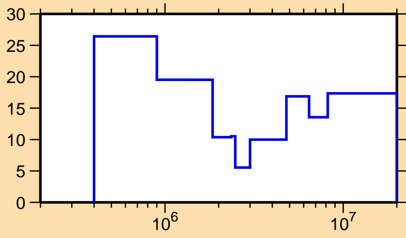
\Delta\sigma/\sigma vs. E for ^{167}\text{Ta}(n,\text{nonel.})
