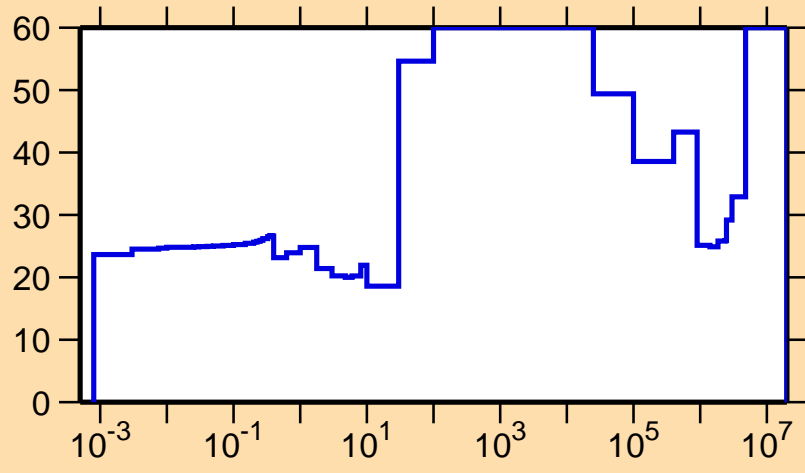
\Delta\sigma/\sigma vs. E for ^{167}\text{Ta}(n,\text{el.})
