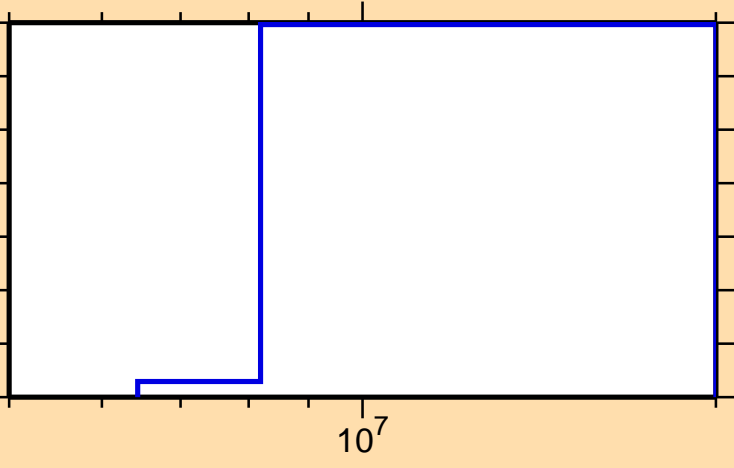
\sigma vs. E for ^{167}\text{Ta} (mt 45)
