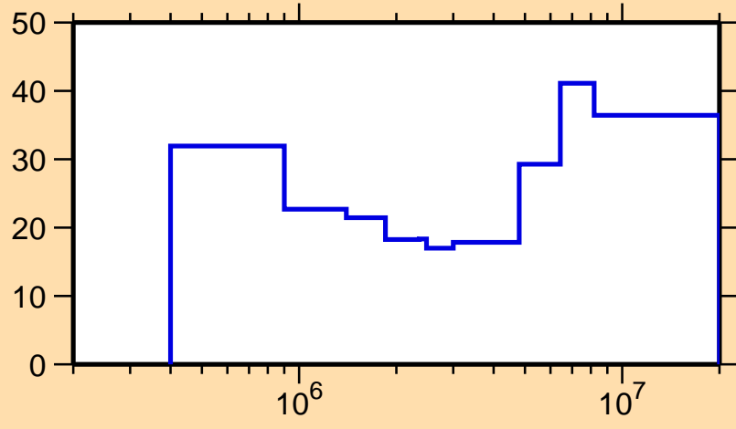
\Delta\sigma/\sigma vs. E for ^{167}\text{Ta}(n,\text{tot.})
