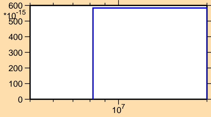
\sigma vs. E for ^{167}\text{Ta}(n,\text{pt})
