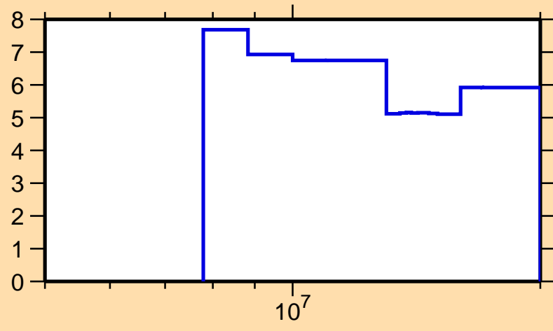
\Delta\sigma/\sigma vs. E for ^{168}\text{Ta}(n,\text{nonel.})
