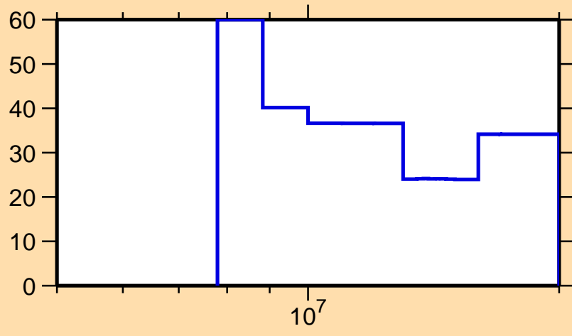
\Delta\sigma/\sigma vs. E for ^{168}\text{Ta}(n,2n)
