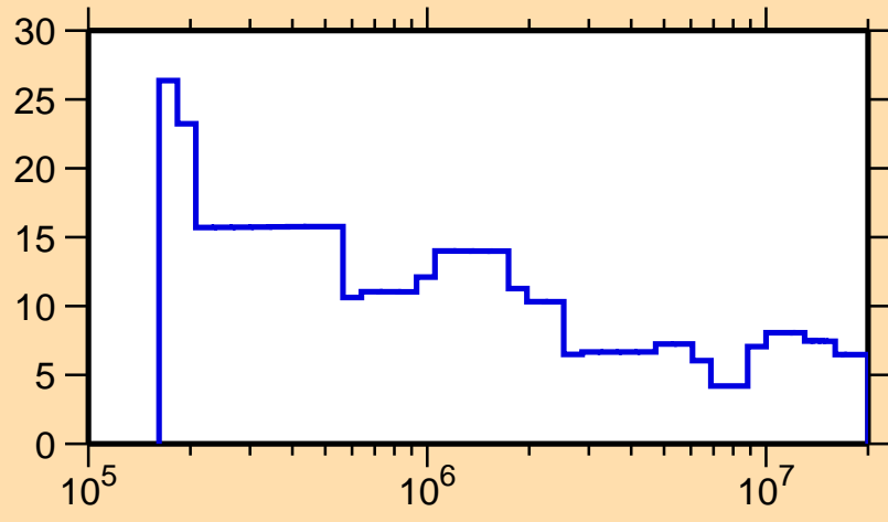
\Delta\sigma/\sigma vs. E for ^{168}\text{Ta}(n,\text{el.})
