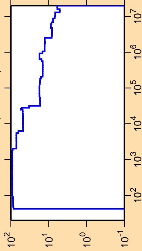
\Delta\sigma/\sigma vs. E for ^{168}\text{Ta}(n,\text{nonel.})
