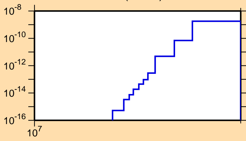
\sigma vs. E for ^{168}\text{Ta} (mt 34)
