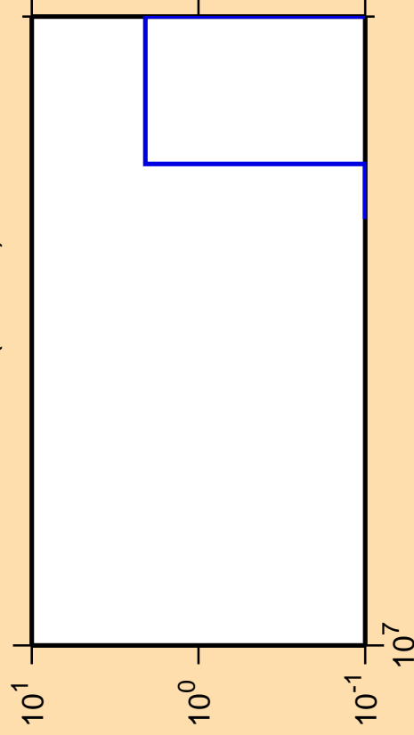
\Delta\sigma/\sigma vs. E for ^{168}\text{Ta}(n,3n\alpha)
