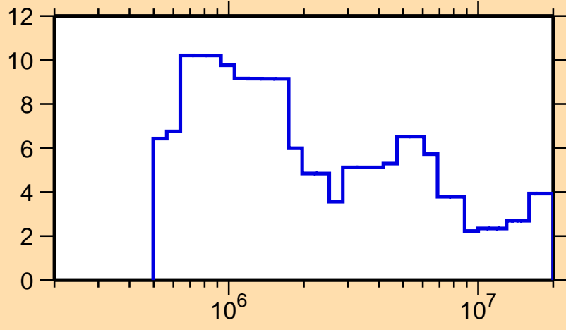
\Delta\sigma/\sigma vs. E for ^{168}\text{Ta}(n,\text{tot.})
