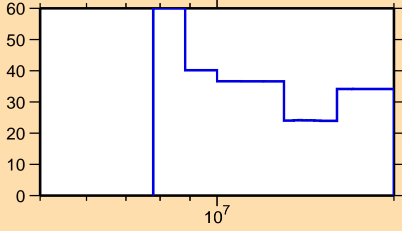
\Delta\sigma/\sigma vs. E for ^{168}\text{Ta}(n,2n)
