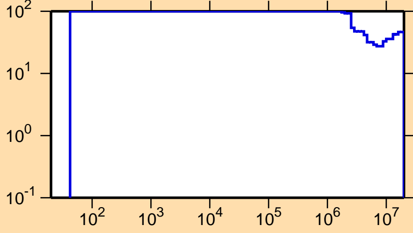
\Delta\sigma/\sigma vs. E for ^{168}\text{Ta}(n,p)
