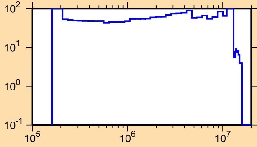
\Delta\sigma/\sigma vs. E for ^{168}\text{Ta}(n,n_1)
