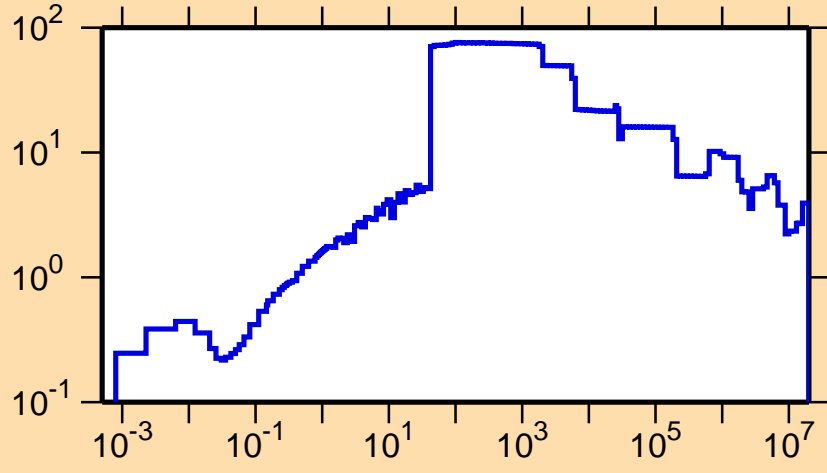
\Delta\sigma/\sigma vs. E for ^{168}\text{Ta}(n,\text{tot.})
