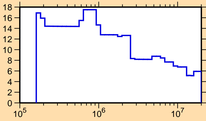
\Delta\sigma/\sigma vs. E for ^{168}\text{Ta}(n,\text{nonel.})
