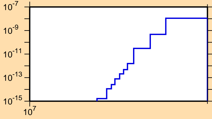
\sigma vs. E for ^{168}\text{Ta}(n,\text{pt})
