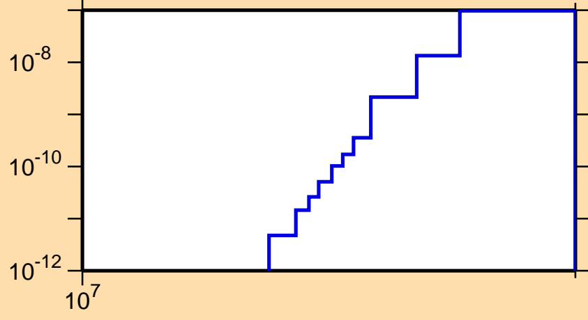
\sigma vs. E for ^{168}\text{Ta}(n,pd)
