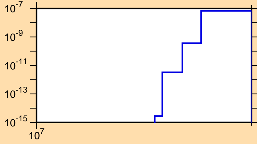
\sigma vs. E for ^{168}\text{Ta}(n,nt)
