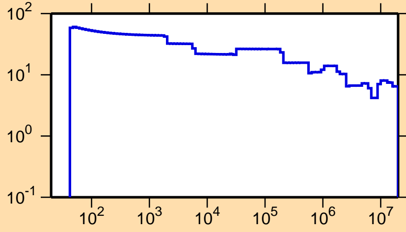
\Delta\sigma/\sigma vs. E for ^{168}\text{Ta}(n,\text{el.})
