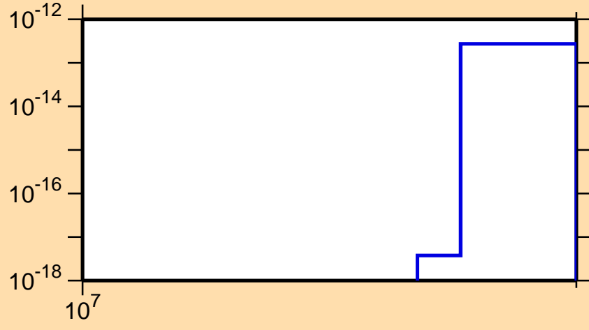
\sigma vs. E for ^{168}\text{Ta}(n,3n\alpha)
