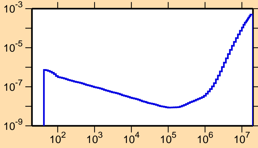
\sigma vs. E for ^{168}\text{Ta}(n,p\alpha)
