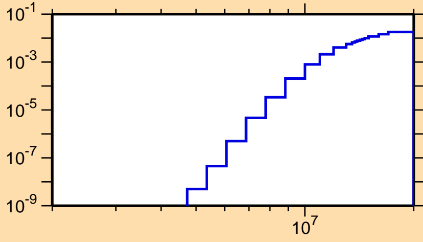
\sigma vs. E for ^{168}\text{Ta}(n,d)
