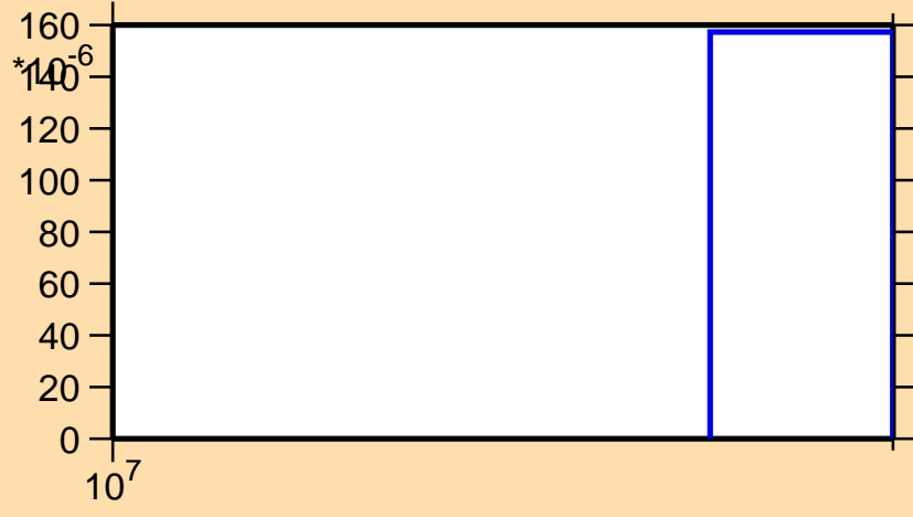
\sigma vs. E for ^{168}\text{Ta}(n,3n)
