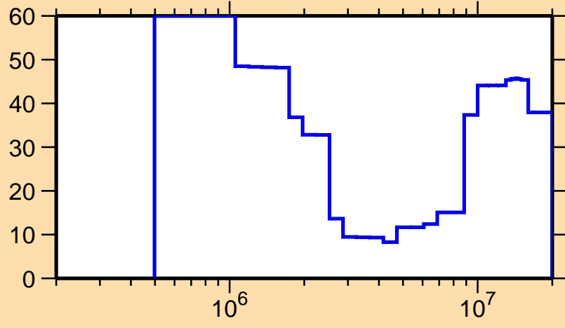
\Delta\sigma/\sigma vs. E for ^{168}\text{Ta}(n,\text{inel.})
