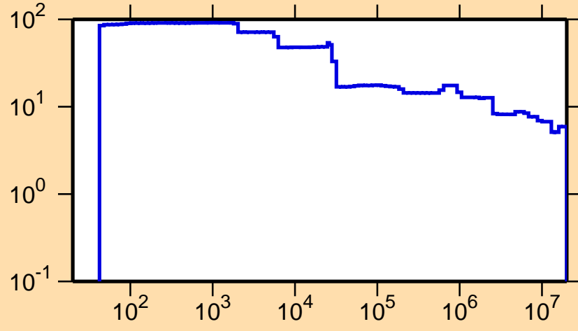
\Delta\sigma/\sigma vs. E for ^{168}\text{Ta}(n,\text{nonel.})
