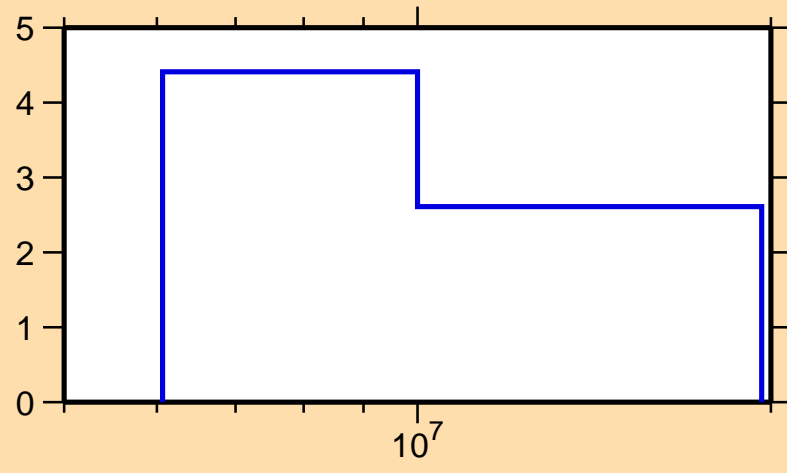
\Delta\sigma/\sigma vs. E for ^{168}\text{Ta}(n,\text{tot.})
