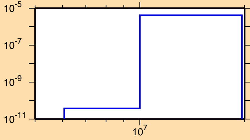
\sigma vs. E for ^{168}\text{Ta}(\text{mt } 45)
