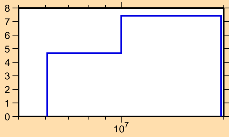
\Delta\sigma/\sigma vs. E for ^{168}\text{Ta}(n,\text{el.})
