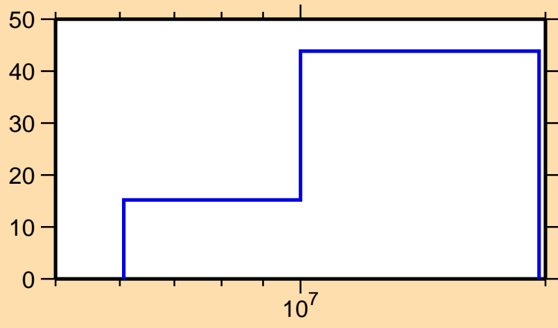
\Delta\sigma/\sigma vs. E for ^{168}\text{Ta}(n,\text{inel.})
