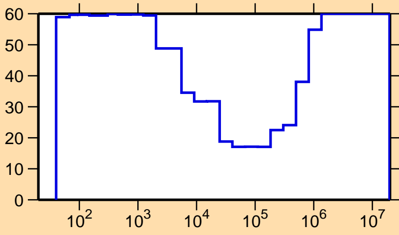
\Delta\sigma/\sigma vs. E for ^{168}\text{Ta}(n,\gamma)
