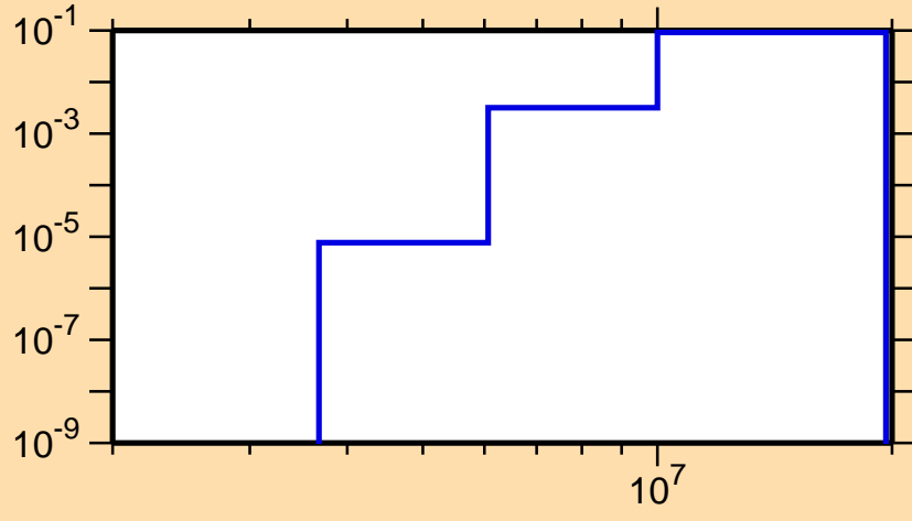
\sigma vs. E for ^{168}\text{Ta}(n,np)
