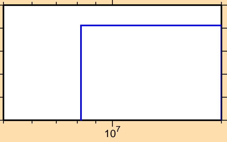
\sigma vs. E for ^{168}\text{Ta}(n,\text{nd})
