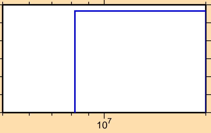
\sigma vs. E for ^{168}\text{Ta}(n,nt)
