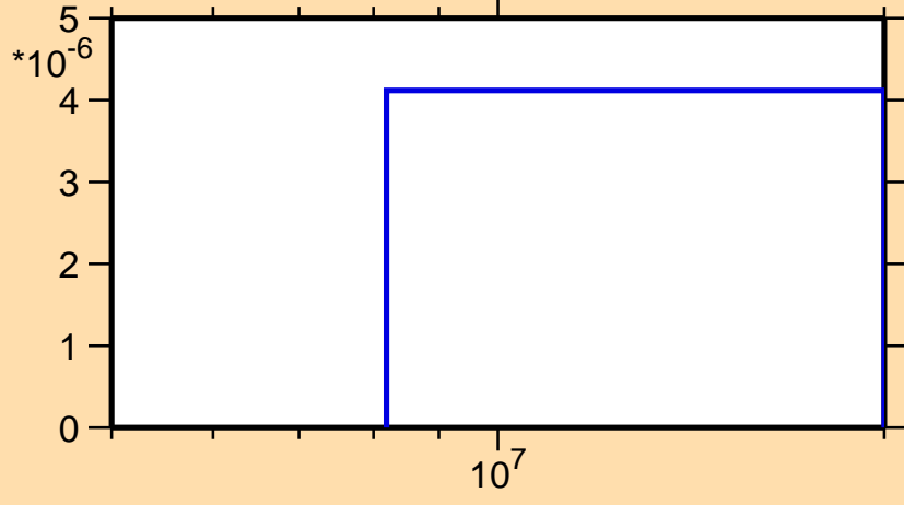
\sigma vs. E for ^{168}\text{Ta}(n,\text{nd})
