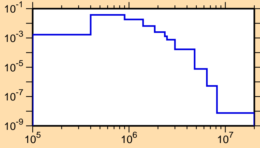
\sigma vs. E for ^{168}\text{Ta}(n,n_2)
