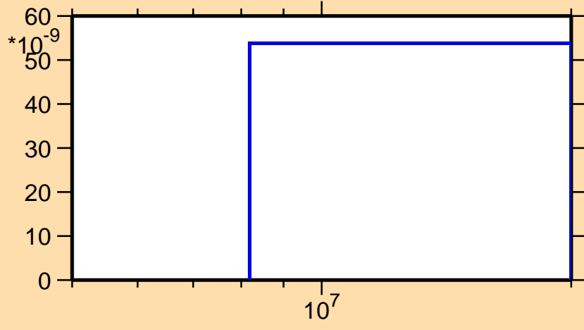
\sigma vs. E for ^{168}\text{Ta}(\text{mt117})
