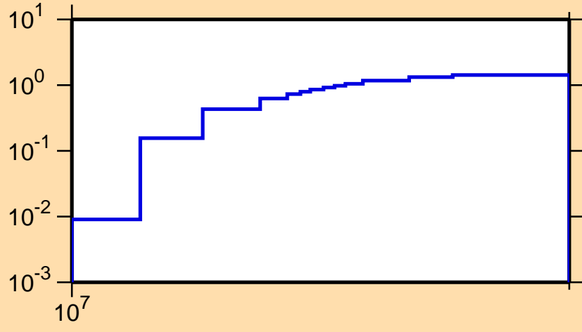
\sigma vs. E for ^{169}\text{Ta}(n,2n)
