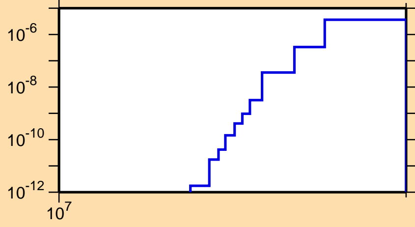
\sigma vs. E for ^{169}\text{Ta}(n,\text{nd})
