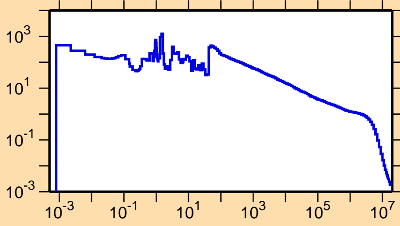
\sigma vs. E for ^{169}\text{Ta}(n,\gamma)
