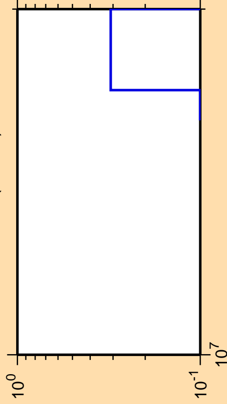
\Delta\sigma/\sigma vs. E for ^{169}\text{Ta}(n,3n\alpha)
