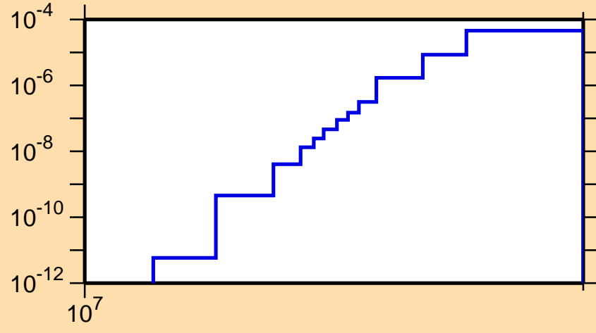
\sigma vs. E for ^{169}\text{Ta}(n,2n\alpha)
