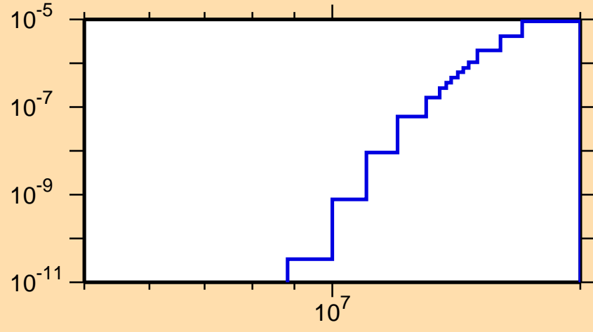
\sigma vs. E for ^{169}\text{Ta} (mt 45)
