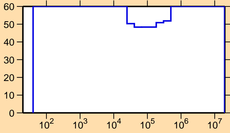
\Delta\sigma/\sigma vs. E for ^{169}\text{Ta}(n,\gamma)
