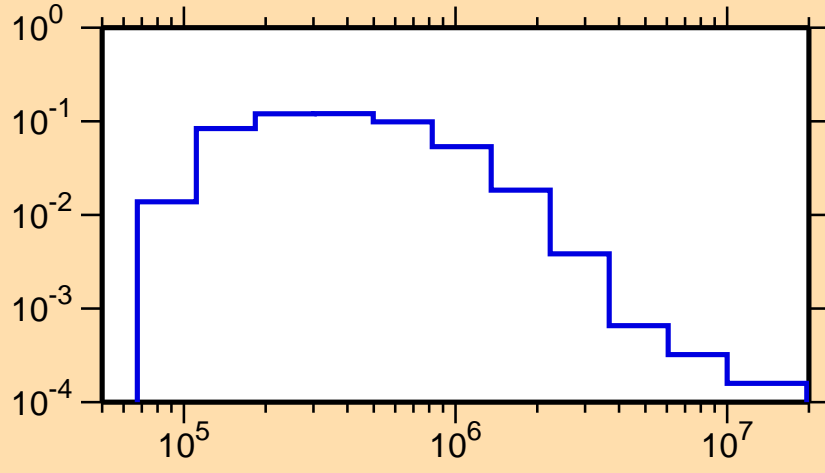
\sigma vs. E for ^{169}\text{Ta}(n,n_3)
