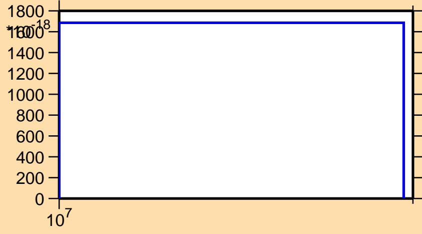
\sigma vs. E for ^{169}\text{Ta}(n,3n\alpha)
