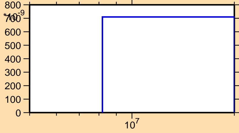
\sigma vs. E for ^{169}\text{Ta} (mt 45)
