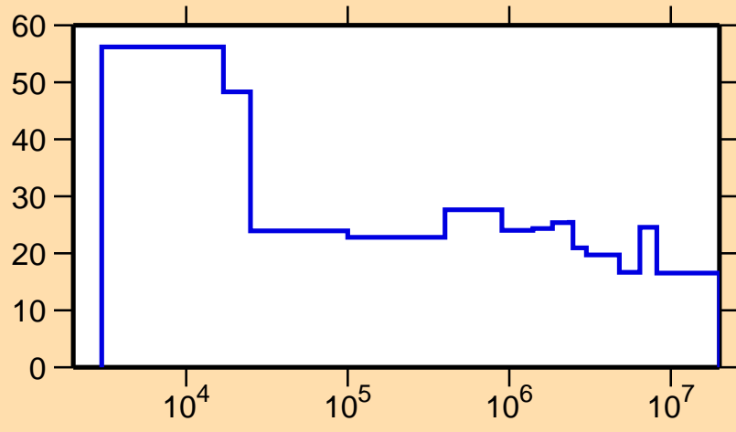
\Delta\sigma/\sigma vs. E for ^{169}\text{Ta}(n,\text{tot.})
