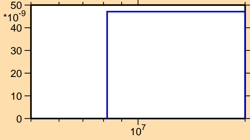
\sigma vs. E for ^{169}\text{Ta}(n,\text{nd})
