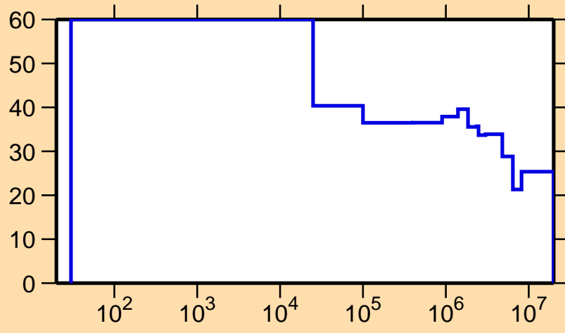
\Delta\sigma/\sigma vs. E for ^{169}\text{Ta}(n,\text{nonel.})
