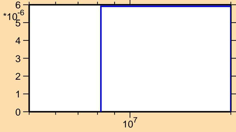
\sigma vs. E for ^{169}\text{Ta}(n,3n)
