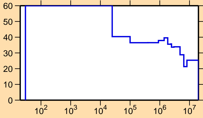
\Delta\sigma/\sigma vs. E for ^{169}\text{Ta}(n,\text{nonel.})
