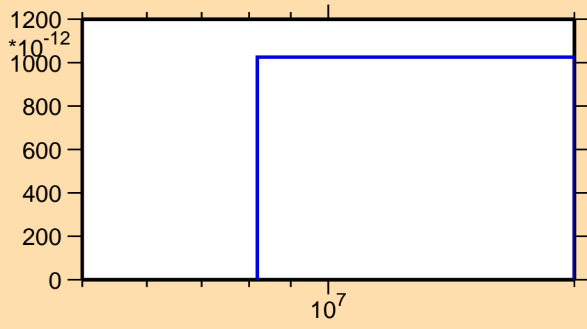
\sigma vs. E for ^{169}\text{Ta}(n,nt)
