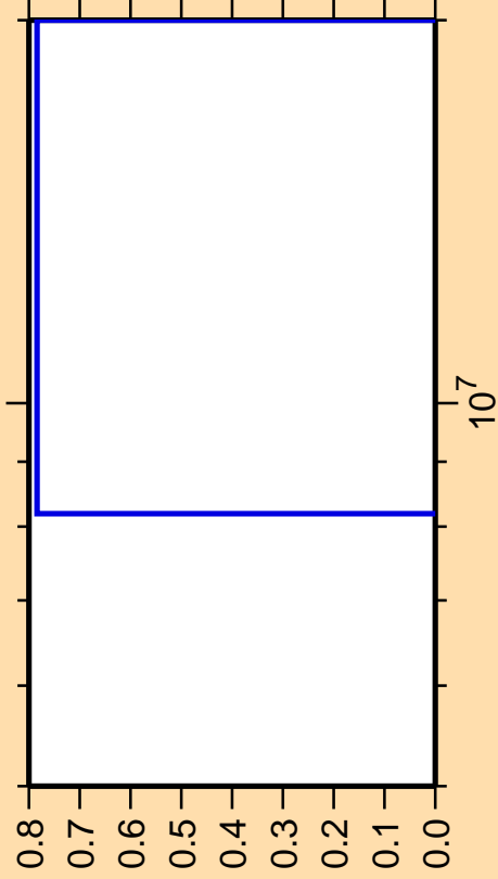
\Delta\sigma/\sigma vs. E for ^{169}\text{Ta}(n,\text{pt})
