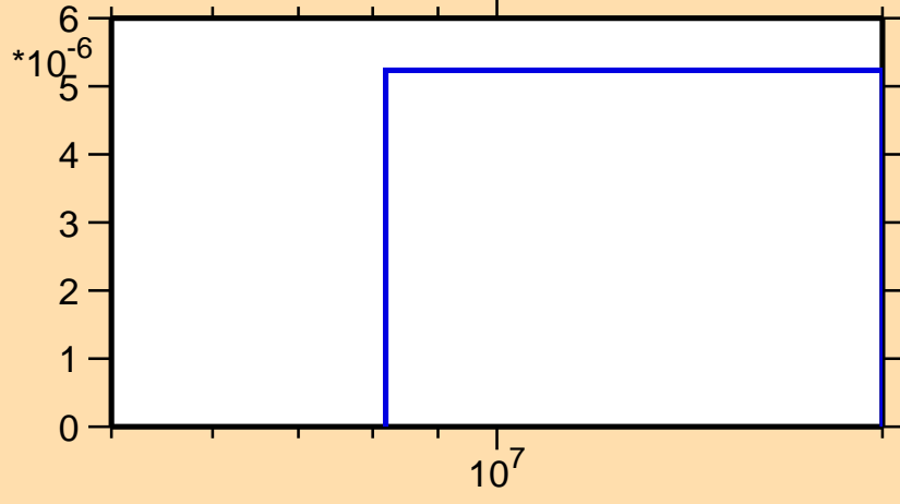
\sigma vs. E for ^{169}\text{Ta}(n,2np)
