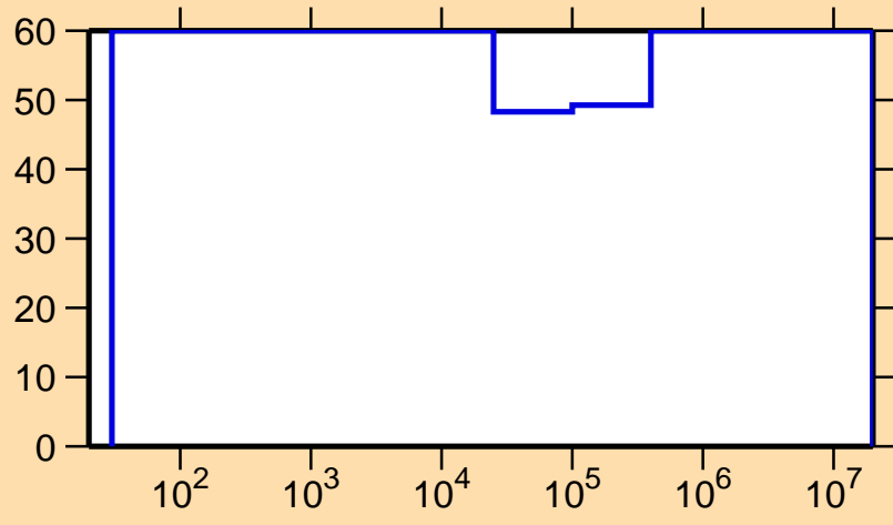
\Delta\sigma/\sigma vs. E for ^{169}\text{Ta}(n,\gamma)
