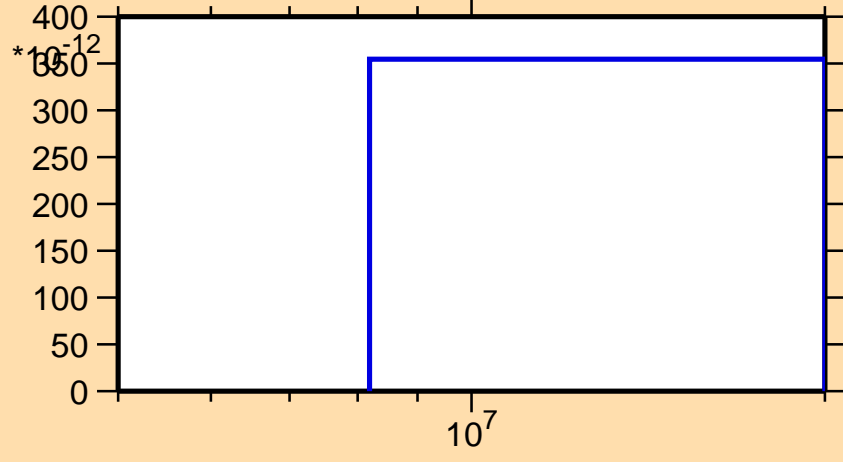
\sigma vs. E for ^{169}\text{Ta}(n,pd)
