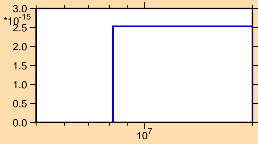
\sigma vs. E for ^{169}\text{Ta}(n,3n\alpha)
