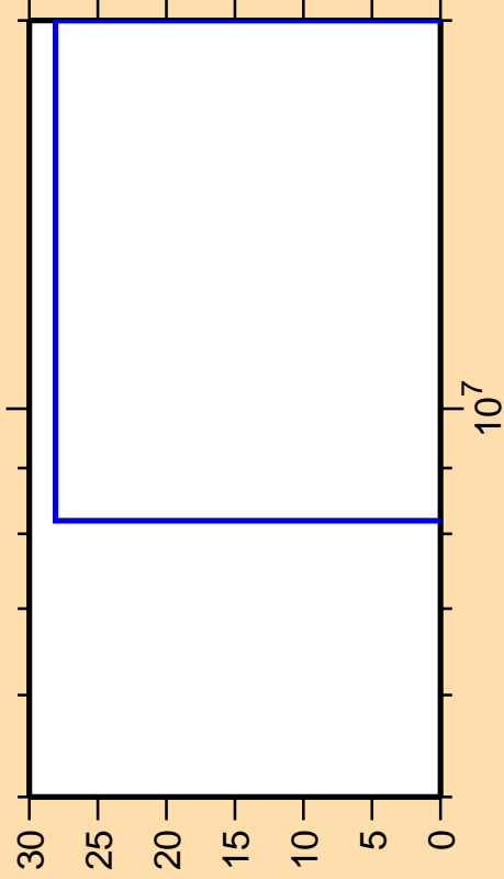
\Delta\sigma/\sigma vs. E for ^{169}\text{Ta}(n,n\text{cont.})
