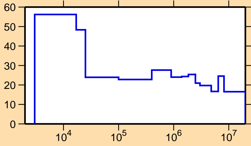
\Delta\sigma/\sigma vs. E for ^{169}\text{Ta}(n,\text{tot.})
