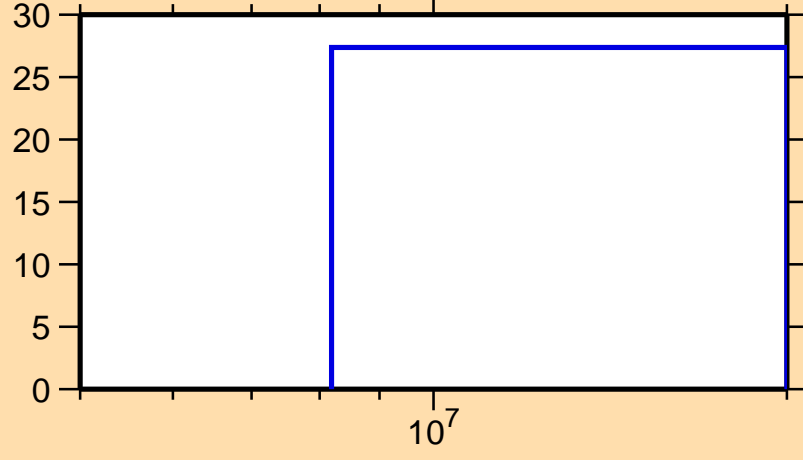
\Delta\sigma/\sigma vs. E for ^{169}\text{Ta}(n,\text{inel.})
