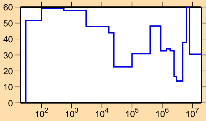
\Delta\sigma/\sigma vs. E for ^{169}\text{Ta}(n,\text{el.})
