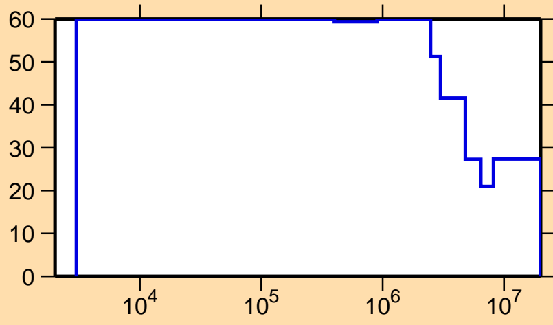
\Delta\sigma/\sigma vs. E for ^{169}\text{Ta}(n,\text{inel.})
