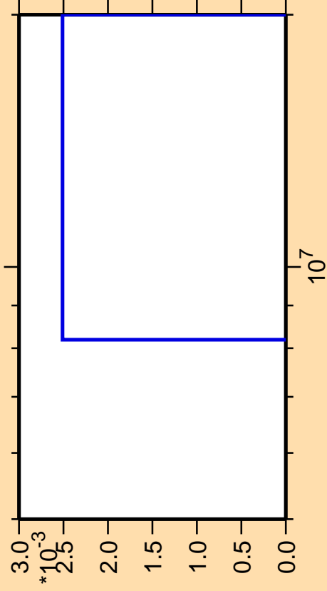
\Delta\sigma/\sigma vs. E for ^{169}\text{Ta}(n,3n\alpha)
