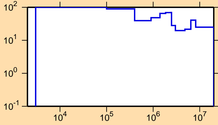
\Delta\sigma/\sigma vs. E for ^{169}\text{Ta}(n,n_1)
