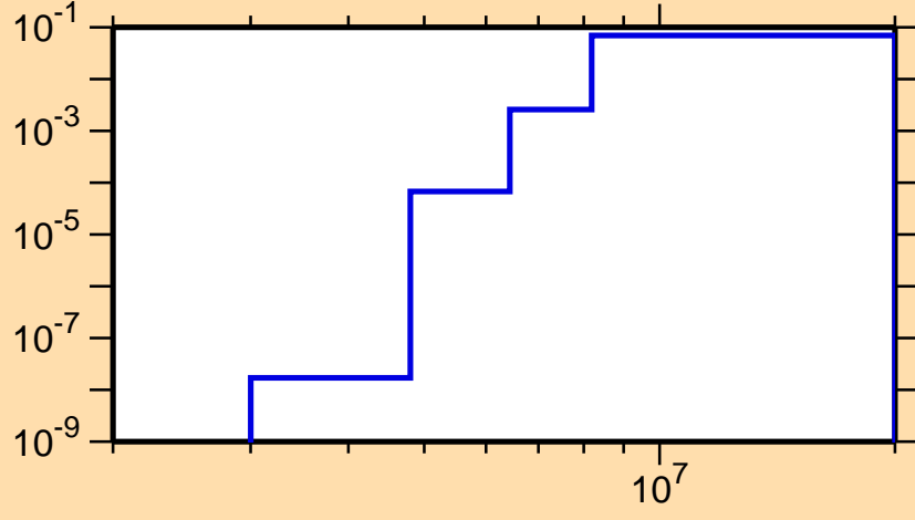
\sigma vs. E for ^{169}\text{Ta}(n,np)
