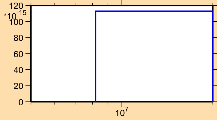
\sigma vs. E for ^{169}\text{Ta}(n,\text{pt})
