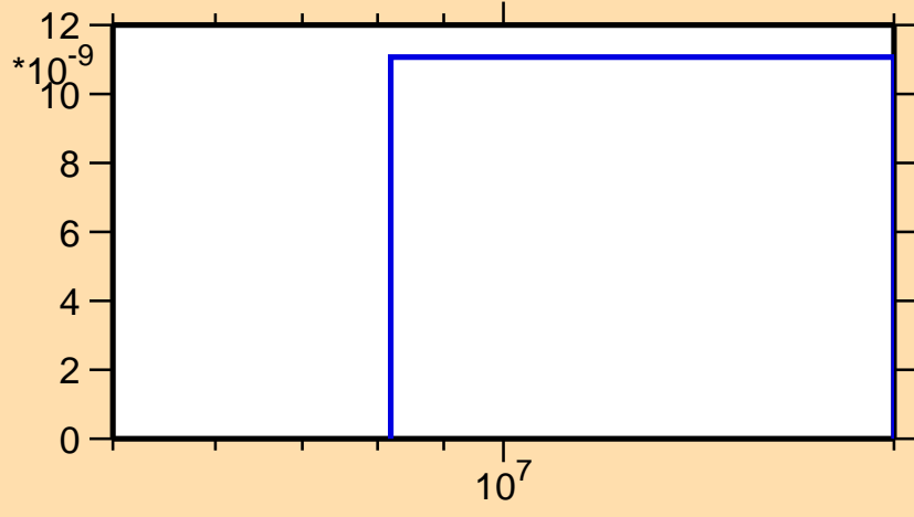
\sigma vs. E for ^{169}\text{Ta}(\text{mt117})
