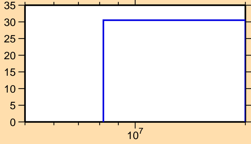
\Delta\sigma/\sigma vs. E for ^{169}\text{Ta}(n,\text{el.})
