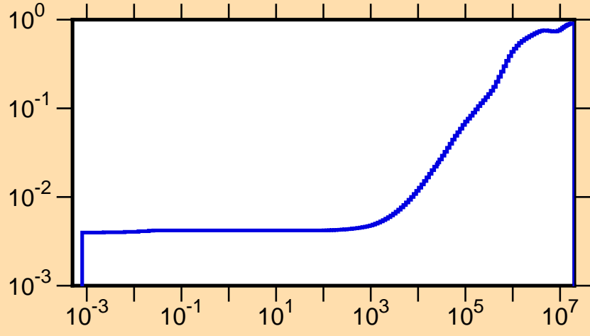
\mu vs. E for ^{170}\text{Ta}(\text{mt251})
