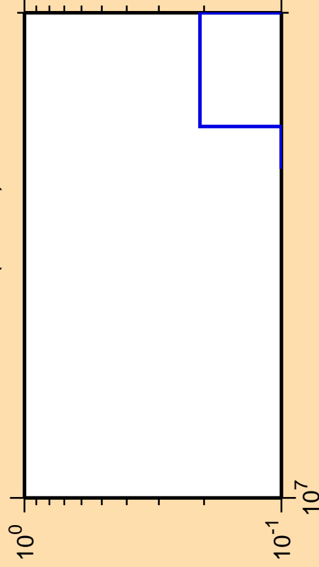
\Delta\sigma/\sigma vs. E for ^{170}\text{Ta}(n,3n\alpha)
