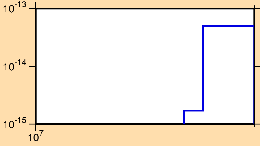
\sigma vs. E for ^{170}\text{Ta}(n,3n\alpha)
