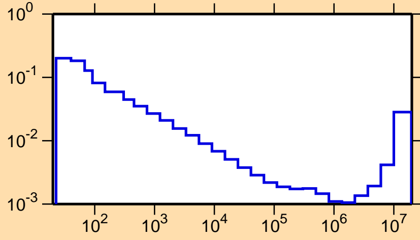
\sigma vs. E for ^{170}\text{Ta}(n,\alpha)
