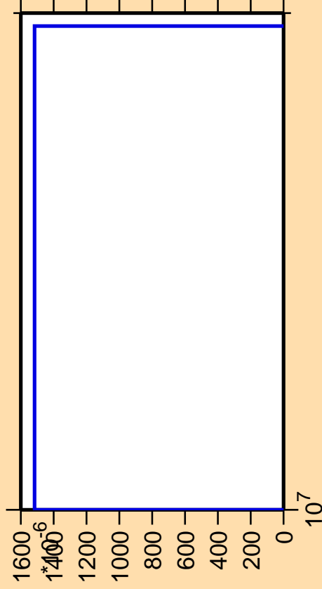
\Delta\sigma/\sigma vs. E for ^{170}\text{Ta}(n,3n\alpha)
