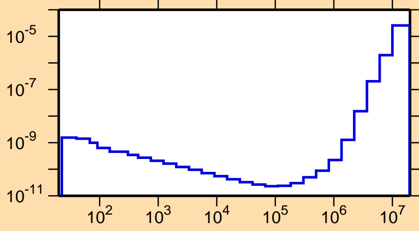
\sigma vs. E for ^{170}\text{Ta}(n,p\alpha)
