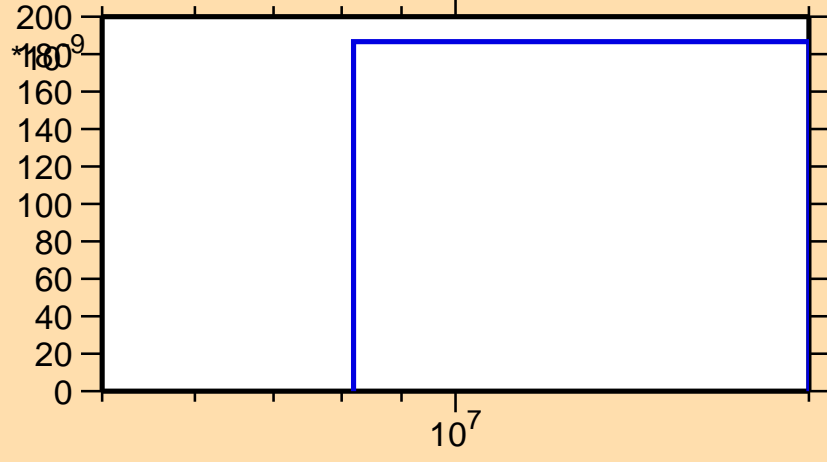
\sigma vs. E for ^{170}\text{Ta} (mt 45)
