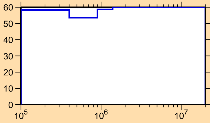
\Delta\sigma/\sigma vs. E for ^{170}\text{Ta}(n,n_1)
