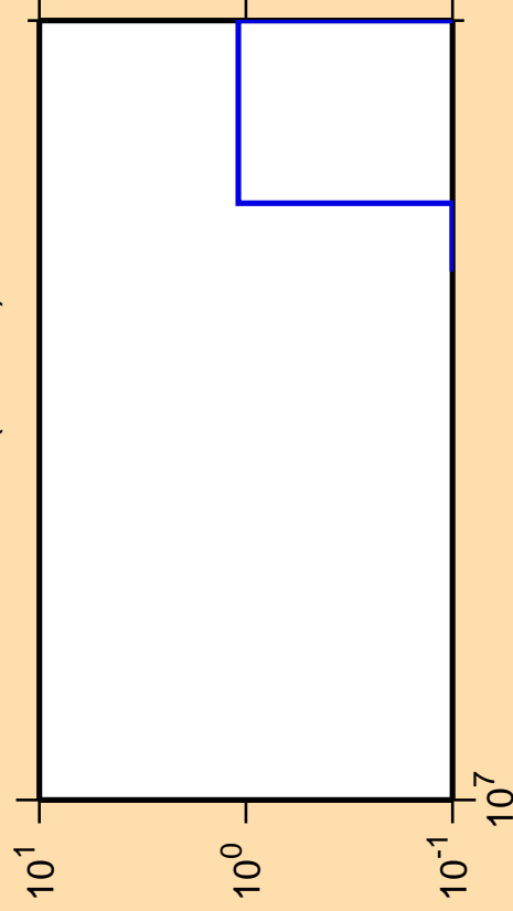
\Delta\sigma/\sigma vs. E for ^{171}\text{Ta}(n,3n\alpha)
