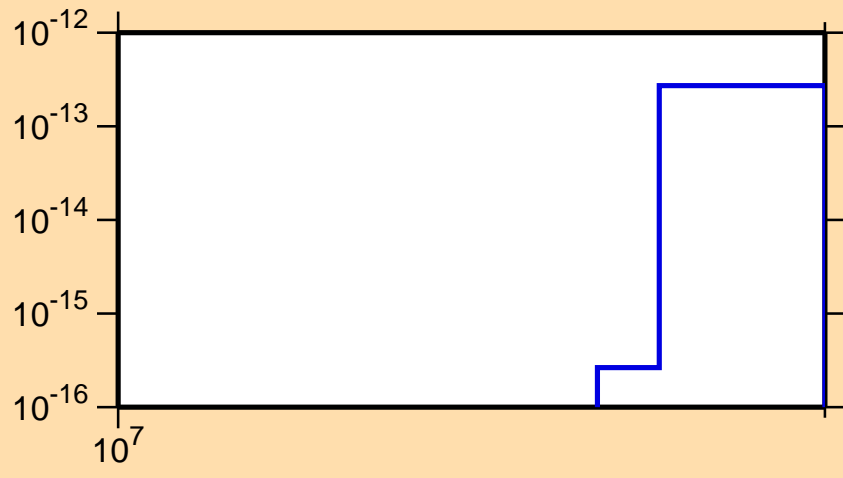
\sigma vs. E for ^{171}\text{Ta}(n,3n\alpha)
