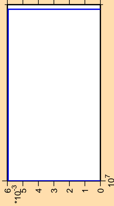
\Delta\sigma/\sigma vs. E for ^{171}\text{Ta}(n,3n\alpha)
