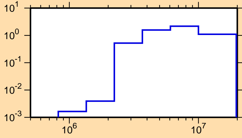
\sigma vs. E for ^{171}\text{Ta}(n,n\text{cont.})
