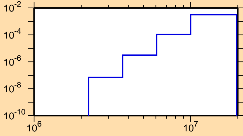
\sigma vs. E for ^{171}\text{Ta}(n,n\alpha)
