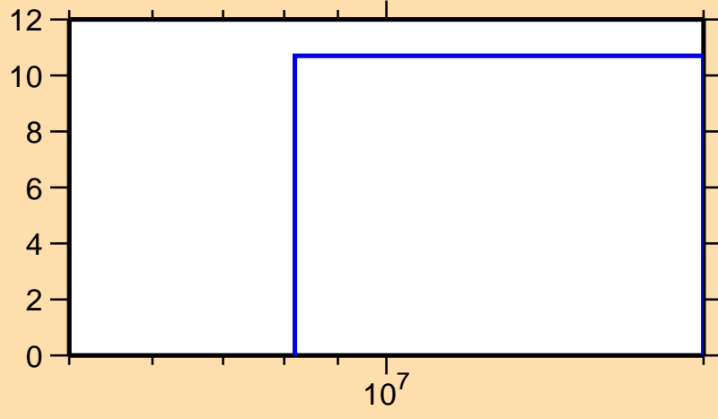
\Delta\sigma/\sigma vs. E for ^{171}\text{Ta}(n,2n)
