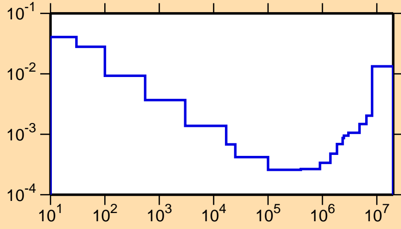
\sigma vs. E for ^{171}\text{Ta}(n,\alpha)
