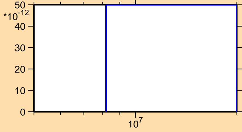
\sigma vs. E for ^{171}\text{Ta}(n,pd)
