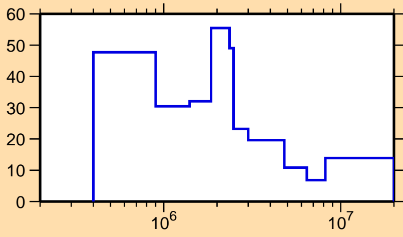
\Delta\sigma/\sigma vs. E for ^{171}\text{Ta}(n,n\text{cont.})
