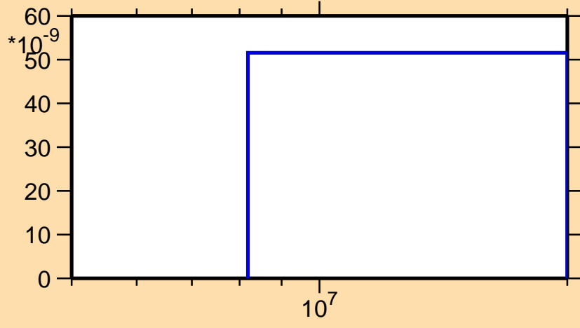
\sigma vs. E for ^{171}\text{Ta} (mt 45)
