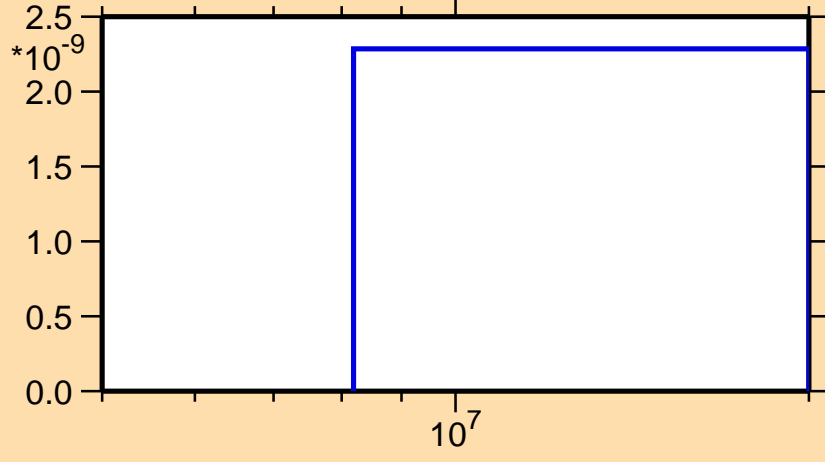
\sigma vs. E for ^{171}\text{Ta}(\text{mt117})
