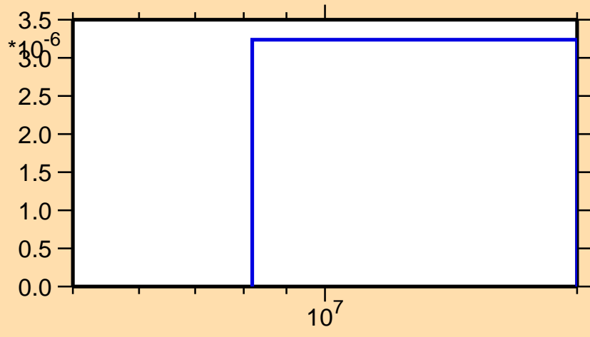
\sigma vs. E for ^{171}\text{Ta}(n,2np)
