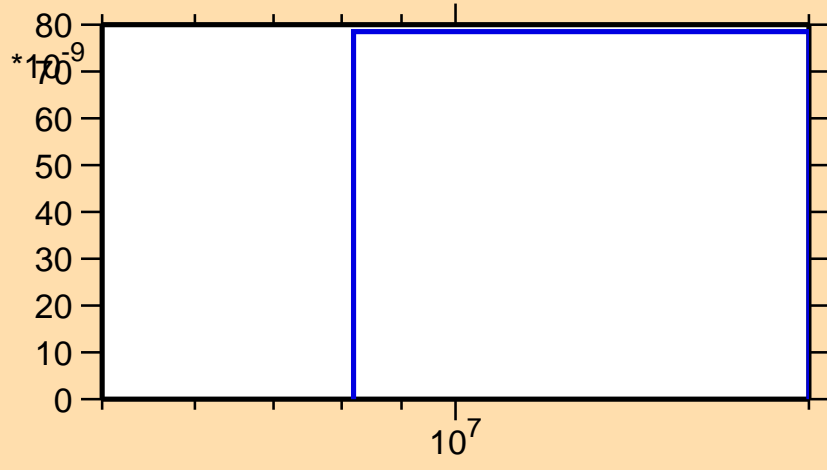
\sigma vs. E for ^{171}\text{Ta}(n,\text{He3})
