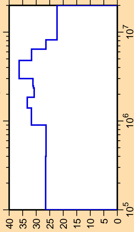
\Delta\sigma/\sigma vs. E for ^{171}\text{Ta}(n,n_3)
