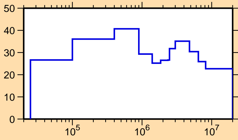
\Delta\sigma/\sigma vs. E for ^{171}\text{Ta}(n,n_1)
