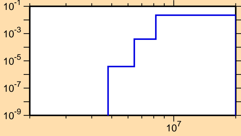
\sigma vs. E for ^{171}\text{Ta}(n,np)
