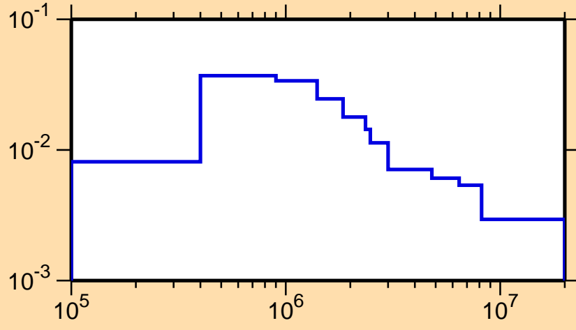
\sigma vs. E for ^{171}\text{Ta}(n,n_3)
