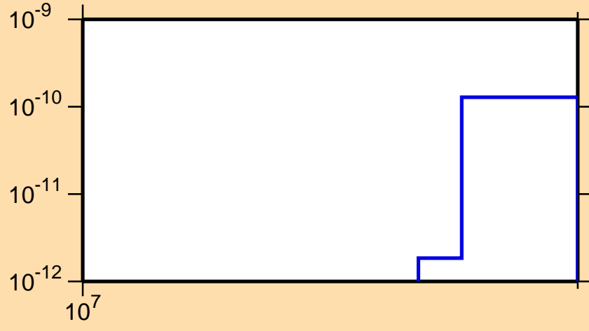
\sigma vs. E for ^{172}\text{Ta} (mt 34)
