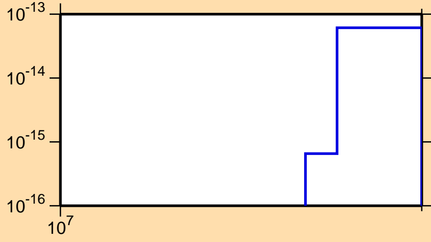
\sigma vs. E for ^{172}\text{Ta}(n,3n\alpha)
