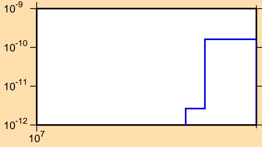
\sigma vs. E for ^{172}\text{Ta}(n,\text{pt})
