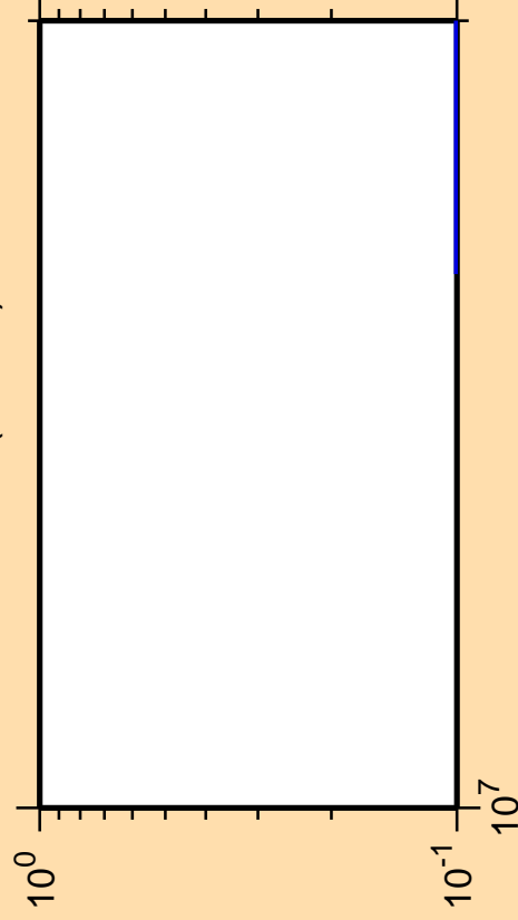
\Delta\sigma/\sigma vs. E for ^{172}\text{Ta}(n,3n\alpha)
