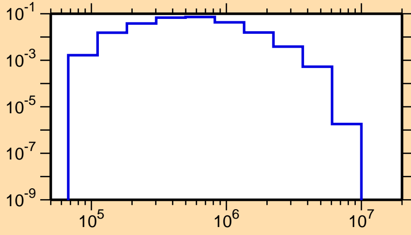
\sigma vs. E for ^{172}\text{Ta}(n,n_3)
