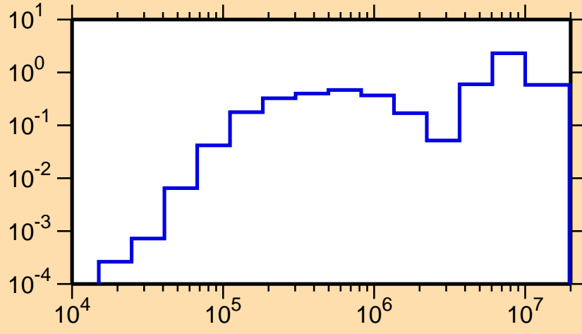
\sigma vs. E for ^{172}\text{Ta}(n,\text{inel.})
