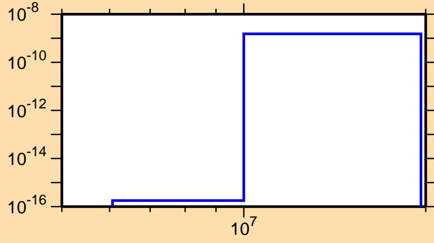
\sigma vs. E for ^{172}\text{Ta}(\text{mt117})
