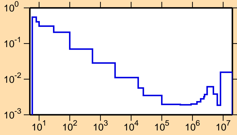
\sigma vs. E for ^{172}\text{Ta}(n,\alpha)
