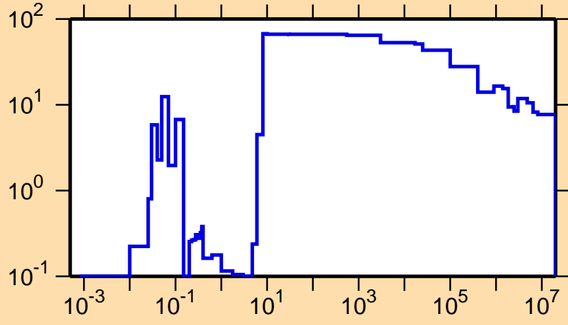
\Delta\sigma/\sigma vs. E for ^{172}\text{Ta}(n,\text{tot.})
