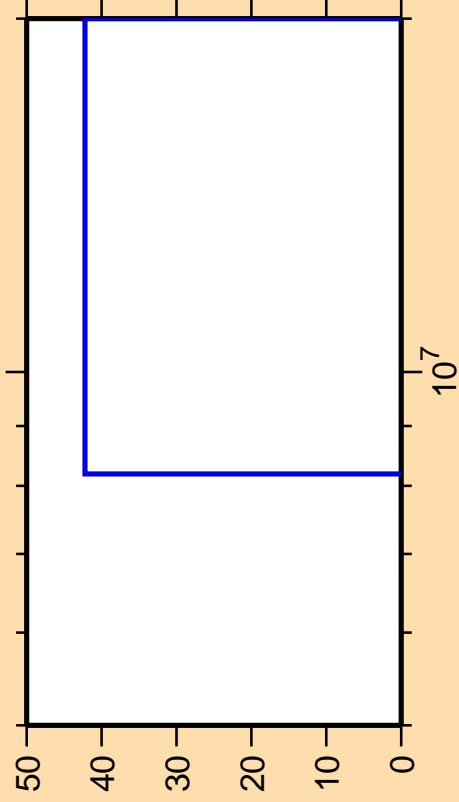
\Delta\sigma/\sigma vs. E for ^{172}\text{Ta}(n,pd)
