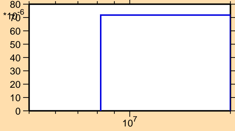
\sigma vs. E for ^{172}\text{Ta}(n,2np)
