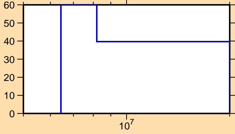
\Delta\sigma/\sigma vs. E for ^{172}\text{Ta}(n,2n)
