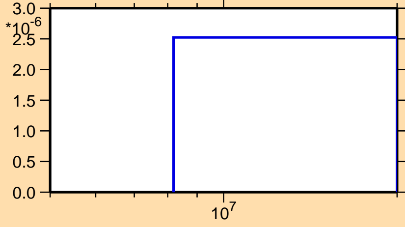
\sigma vs. E for ^{172}\text{Ta}(n,\text{nd})
