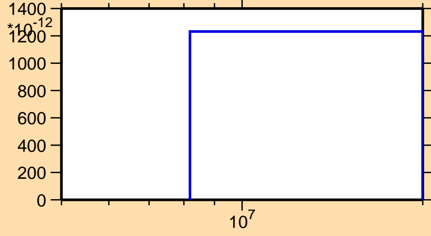
\sigma vs. E for ^{172}\text{Ta}(\text{mt117})
