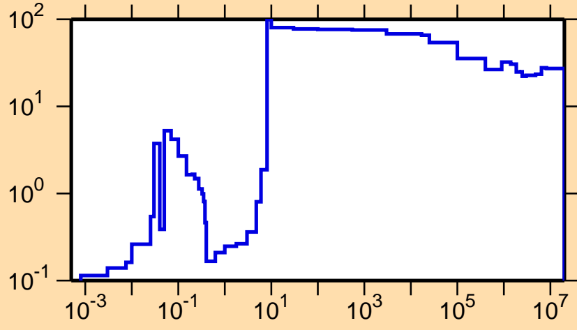
\Delta\sigma/\sigma vs. E for ^{172}\text{Ta}(n,\text{el.})
