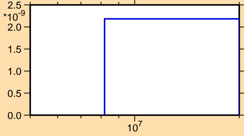
\sigma vs. E for ^{172}\text{Ta}(n,nt)
