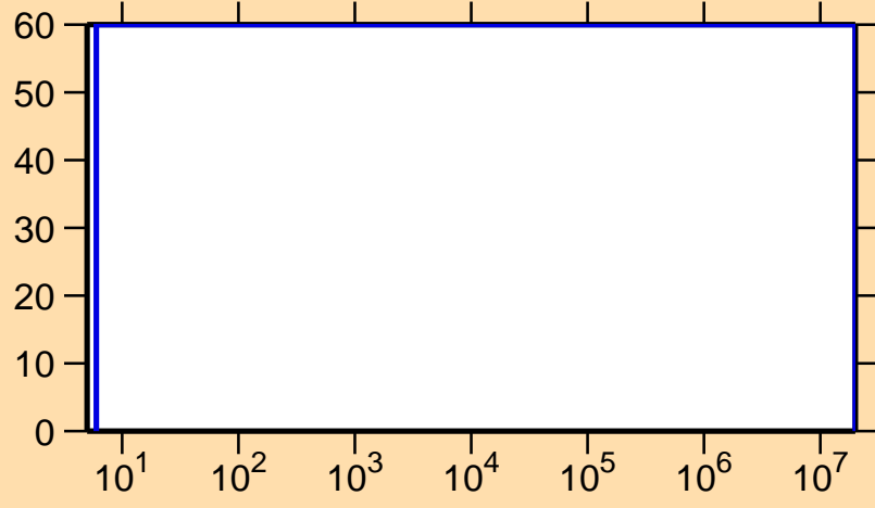
\Delta\sigma/\sigma vs. E for ^{172}\text{Ta}(n,p)
