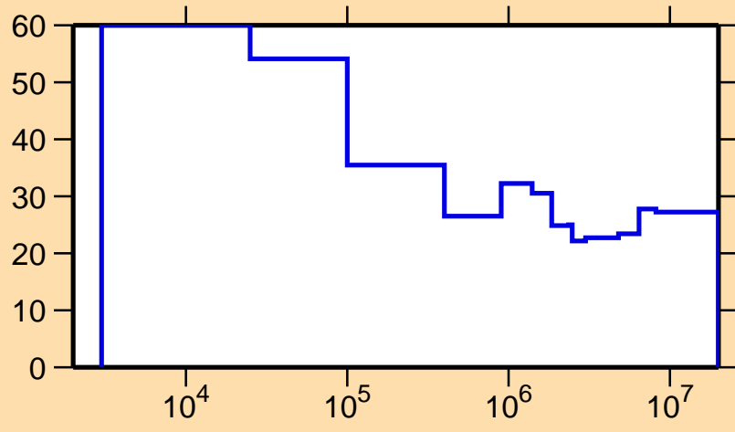
\Delta\sigma/\sigma vs. E for ^{172}\text{Ta}(n,\text{el.})
