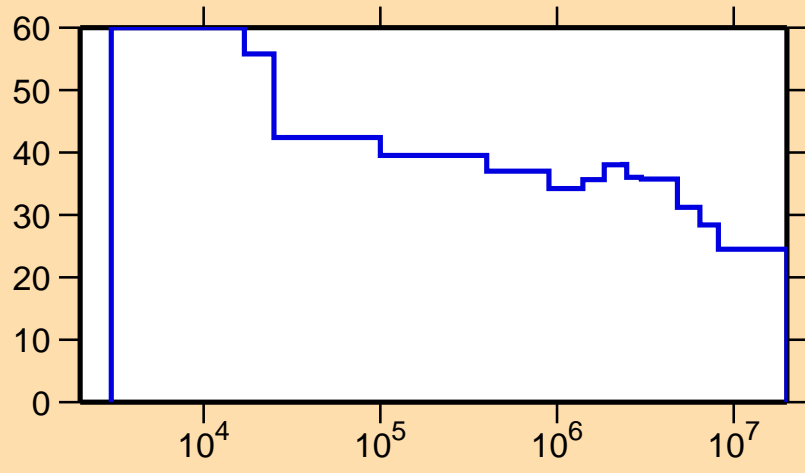
\Delta\sigma/\sigma vs. E for ^{172}\text{Ta}(n,\text{nonel.})
