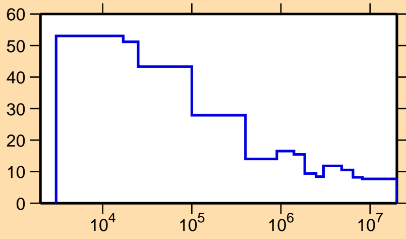
\Delta\sigma/\sigma vs. E for ^{172}\text{Ta}(n,\text{tot.})
