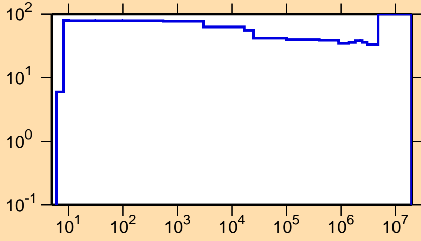
\Delta\sigma/\sigma vs. E for ^{172}\text{Ta}(n,\gamma)
