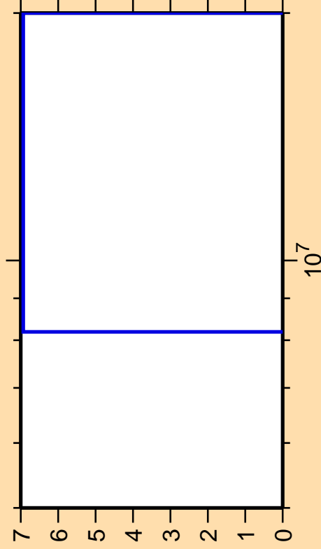
\Delta\sigma/\sigma vs. E for ^{172}\text{Ta}(n,\text{pt})
