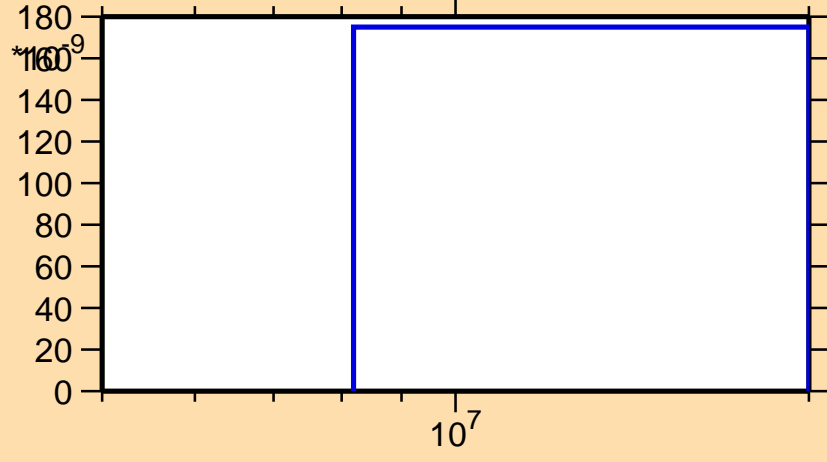
\sigma vs. E for ^{172}\text{Ta}(n,\text{He}3)
