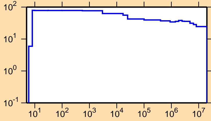
\Delta\sigma/\sigma vs. E for ^{172}\text{Ta}(n,\text{nonel.})
