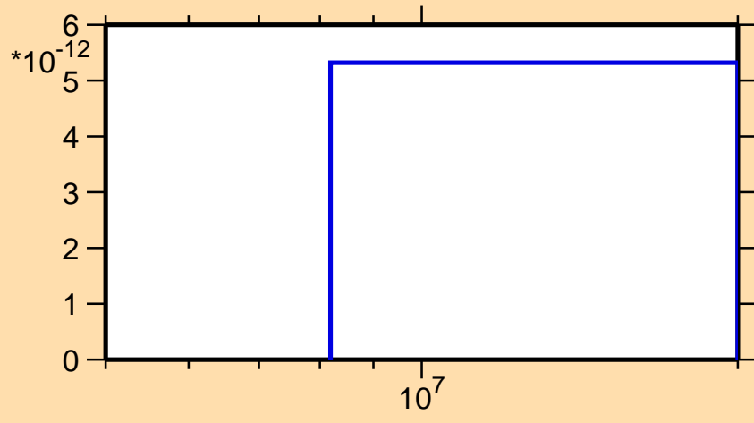
\sigma vs. E for ^{172}\text{Ta}(n,pd)
