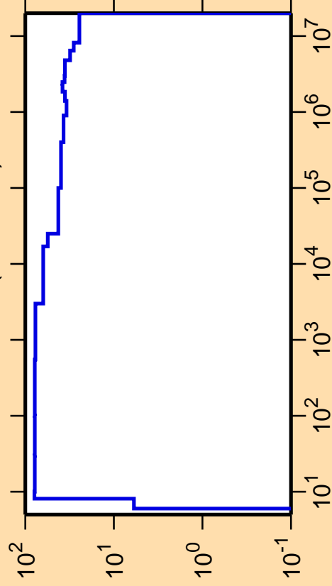
\Delta\sigma/\sigma vs. E for ^{172}\text{Ta}(n,\text{nonel.})
