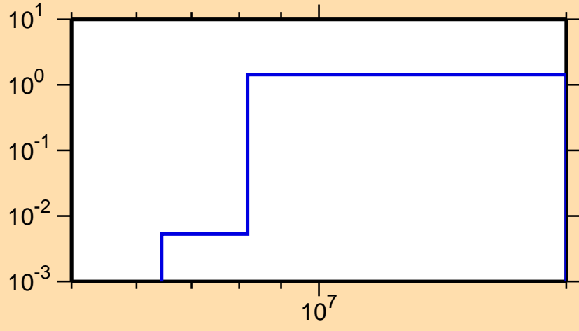
\sigma vs. E for ^{172}\text{Ta}(n,2n)
