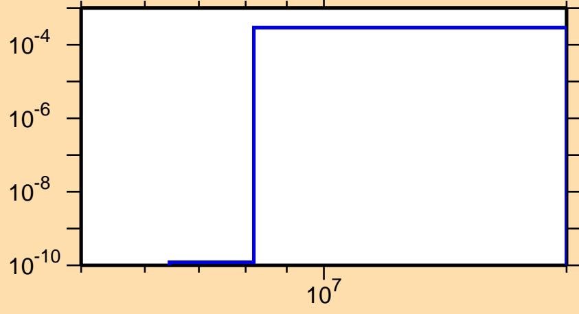
\sigma vs. E for ^{172}\text{Ta}(n,t)
