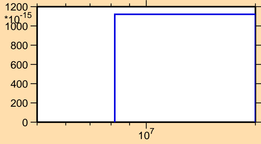
\sigma vs. E for ^{172}\text{Ta} (mt 34)
