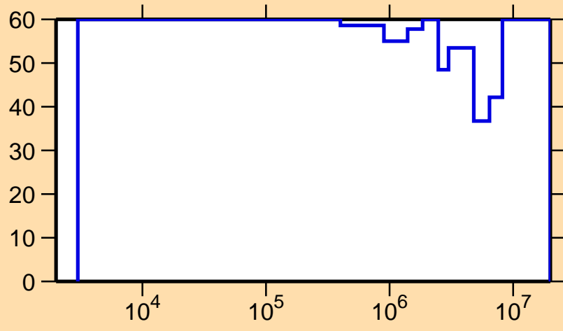
\Delta\sigma/\sigma vs. E for ^{172}\text{Ta}(n,\text{inel.})
