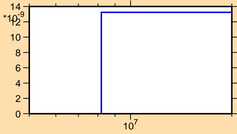
\sigma vs. E for ^{172}\text{Ta} (mt 45)
