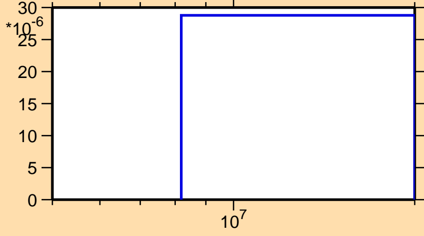
\sigma vs. E for ^{172}\text{Ta}(n,3n)
