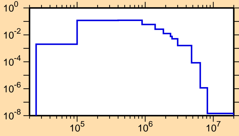
\sigma vs. E for ^{172}\text{Ta}(n,n_4)
