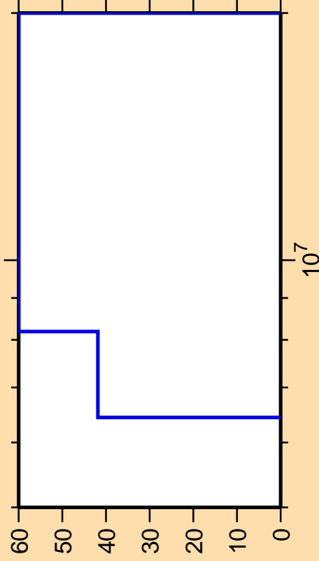
\Delta\sigma/\sigma vs. E for ^{172}\text{Ta}(n,n\text{cont.})
