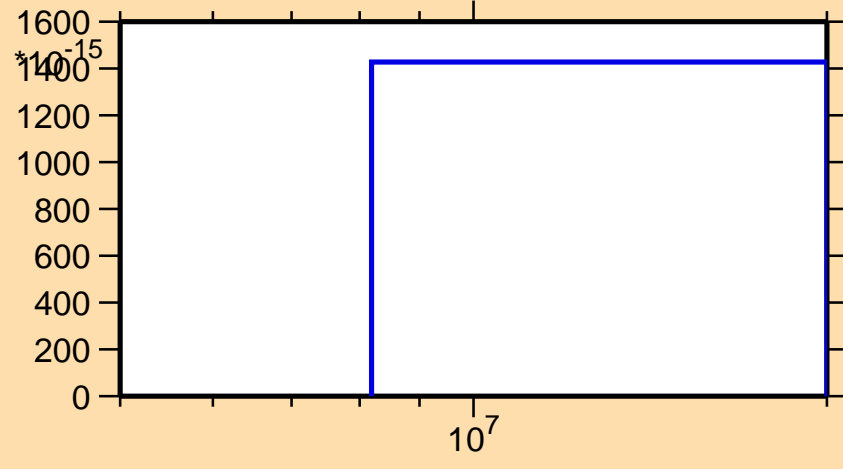
\sigma vs. E for ^{172}\text{Ta}(n,\text{pt})
