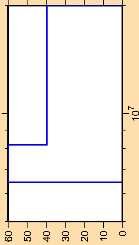
\Delta\sigma/\sigma vs. E for ^{172}\text{Ta}(n,2n)
