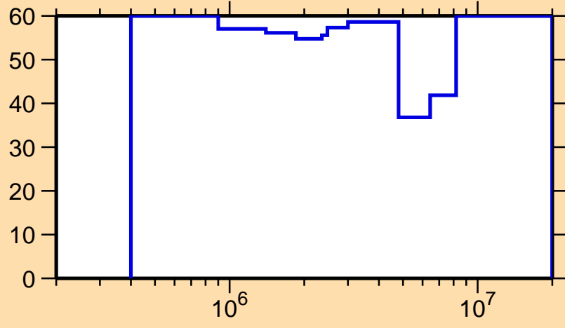
\Delta\sigma/\sigma vs. E for ^{172}\text{Ta}(n,n\text{cont.})
