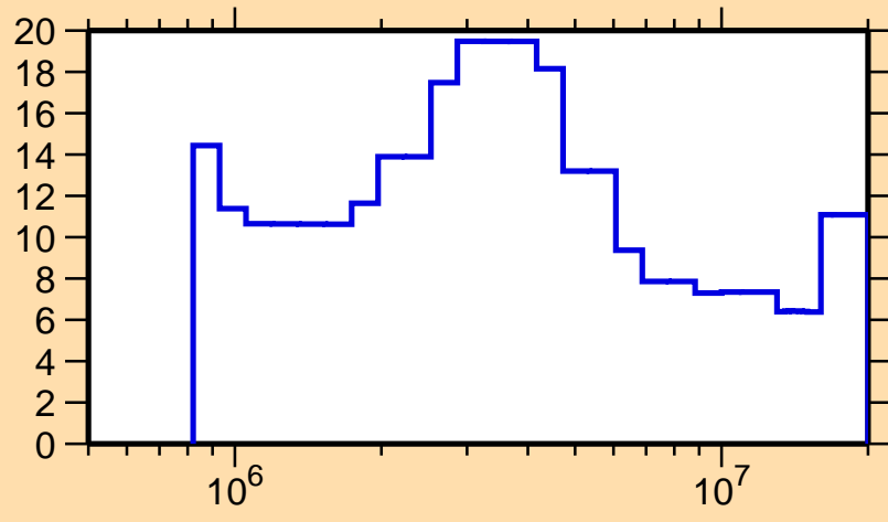
\Delta\sigma/\sigma vs. E for ^{173}\text{Ta}(n,tot.)
