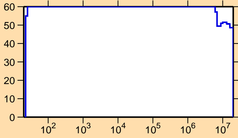
\Delta\sigma/\sigma vs. E for ^{173}\text{Ta}(n,p)
