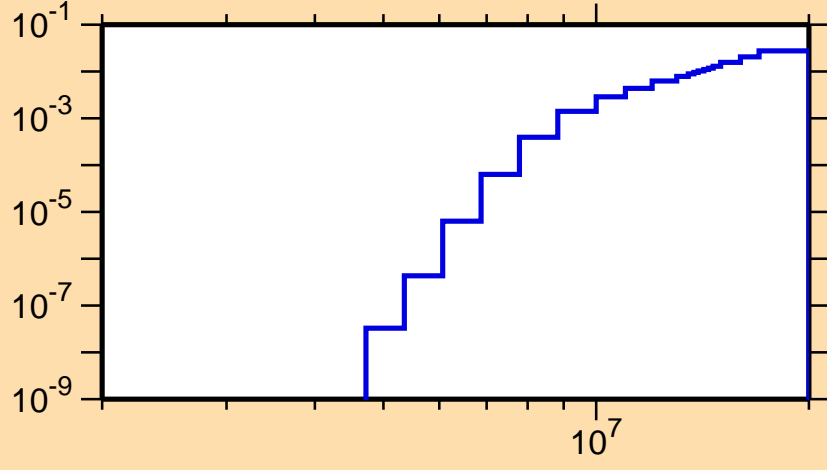
\sigma vs. E for ^{173}\text{Ta}(n,np)
