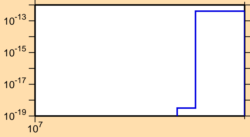
\sigma vs. E for ^{173}\text{Ta}(n,3n\alpha)
