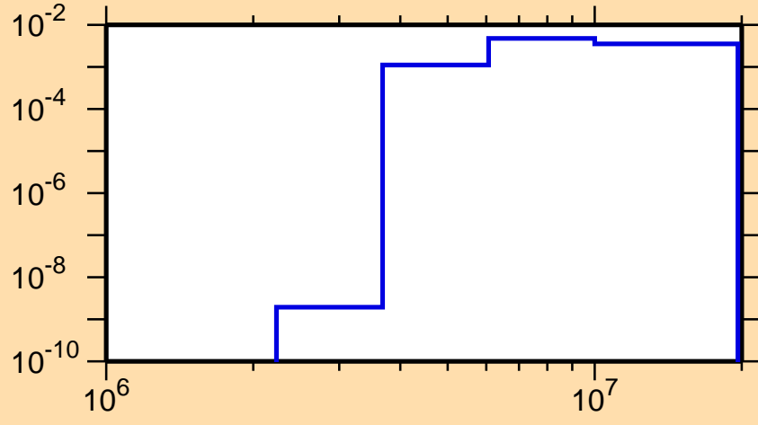
\sigma vs. E for ^{173}\text{Ta}(n,n\alpha)
