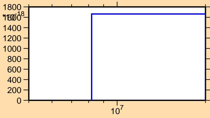
\sigma vs. E for ^{173}\text{Ta}(n,\text{pt})
