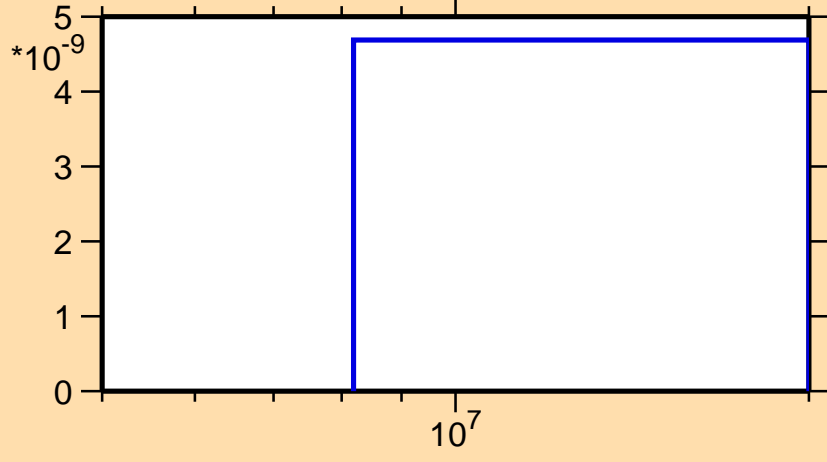
\sigma vs. E for ^{173}\text{Ta}(n,nt)
