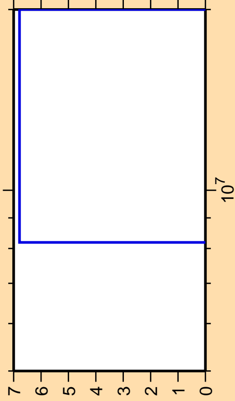
\Delta\sigma/\sigma vs. E for ^{173}\text{Ta}(n,pd)
