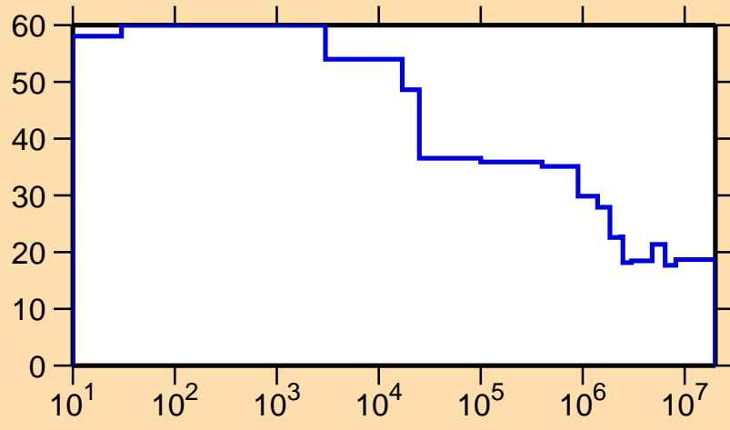
\Delta\sigma/\sigma vs. E for ^{173}\text{Ta}(n,\text{nonel.})
