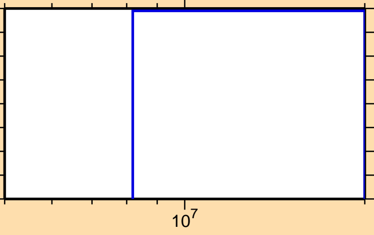
\sigma vs. E for ^{173}\text{Ta}(n,3n)
