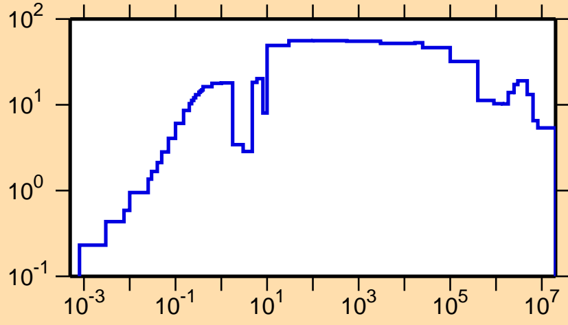
\Delta\sigma/\sigma vs. E for ^{173}\text{Ta}(n,\text{tot.})
