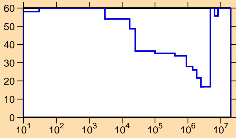
\Delta\sigma/\sigma vs. E for ^{173}\text{Ta}(n,\gamma)
