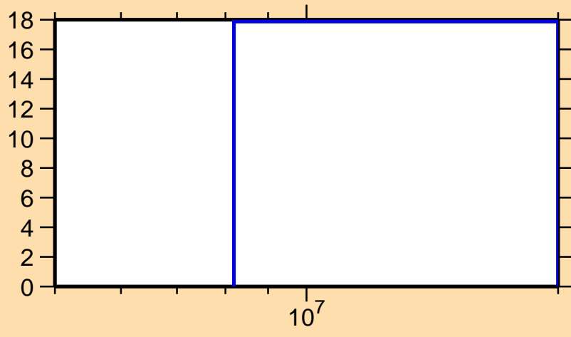
\Delta\sigma/\sigma vs. E for ^{173}\text{Ta}(n,\text{el.})
