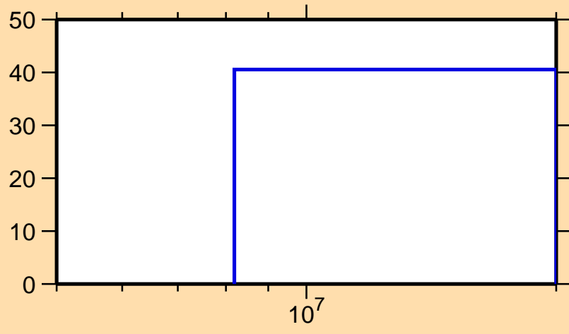
\Delta\sigma/\sigma vs. E for ^{173}\text{Ta}(n,2n)
