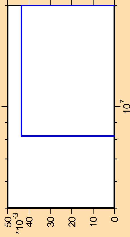
\Delta\sigma/\sigma vs. E for ^{173}\text{Ta} (mt 34)
