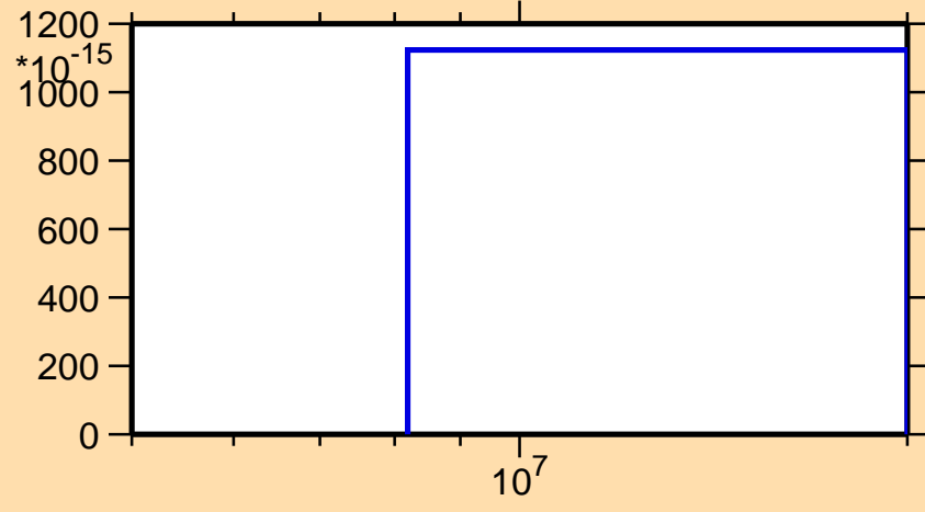
\sigma vs. E for ^{173}\text{Ta}(n,pd)
