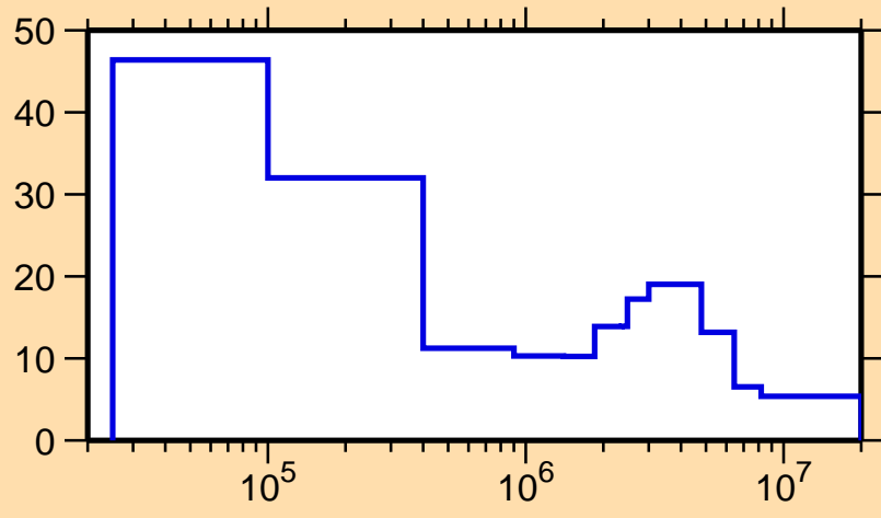
\Delta\sigma/\sigma vs. E for ^{173}\text{Ta}(n,\text{tot.})
