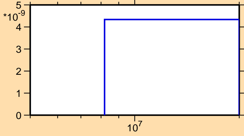
\sigma vs. E for ^{173}\text{Ta} (mt 45)
