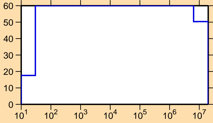
\Delta\sigma/\sigma vs. E for ^{173}\text{Ta}(n,p)
