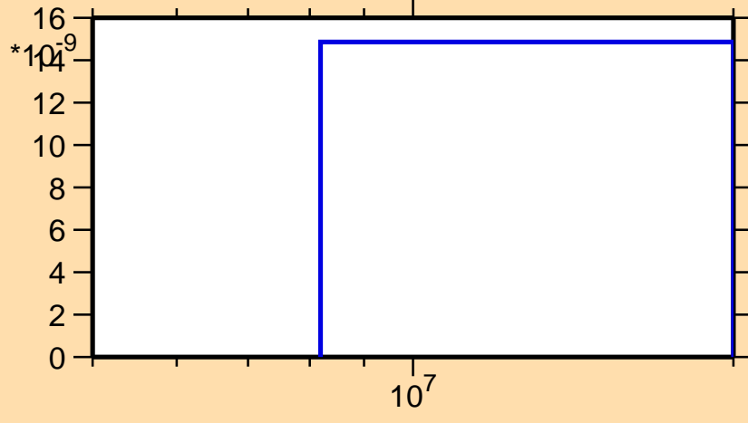
\sigma vs. E for ^{173}\text{Ta}(n,\text{He}3)
