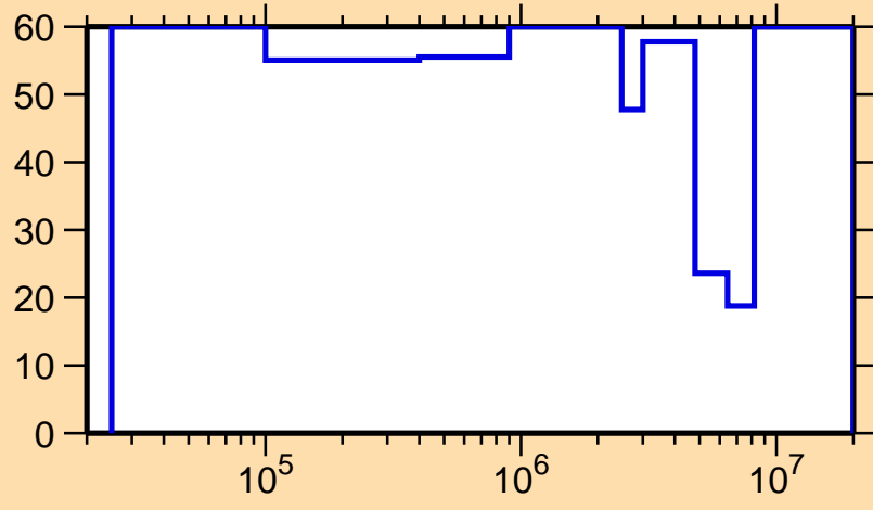
\Delta\sigma/\sigma vs. E for ^{173}\text{Ta}(n,\text{inel.})
