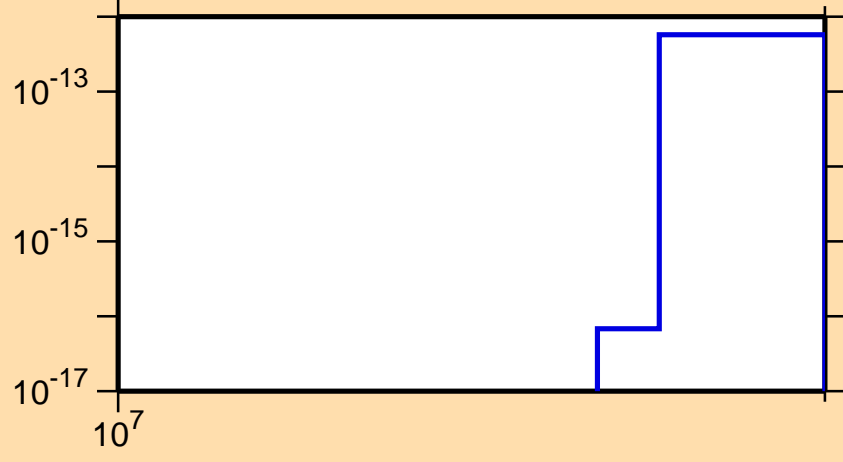
\sigma vs. E for ^{174}\text{Ta}(n,3n\alpha)
