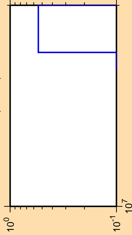
\Delta\sigma/\sigma vs. E for ^{174}\text{Ta}(n,3n\alpha)
