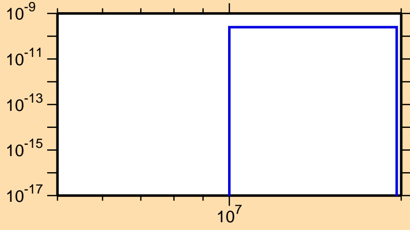
\sigma vs. E for ^{174}\text{Ta}(\text{mt117})
