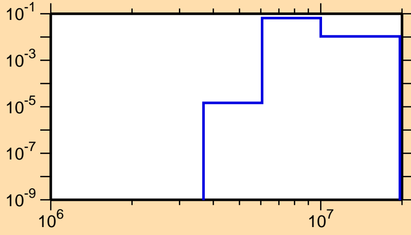
\sigma vs. E for ^{174}\text{Ta}(n,n\alpha)
