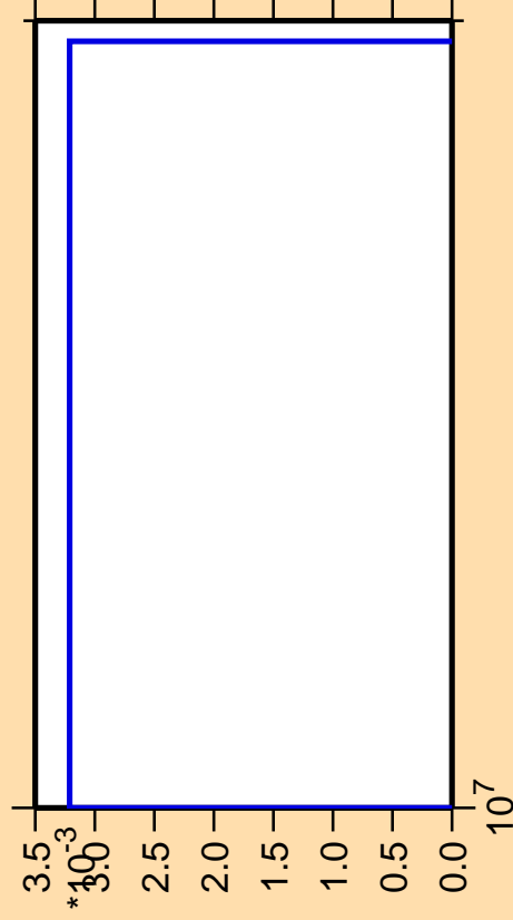
\Delta\sigma/\sigma vs. E for ^{174}\text{Ta}(n,3n\alpha)
