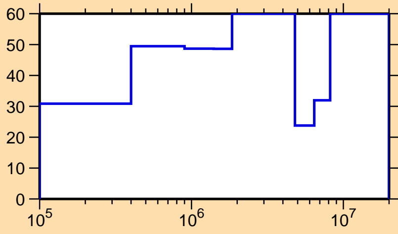
\Delta\sigma/\sigma vs. E for ^{174}\text{Ta}(n,n\text{cont.})
