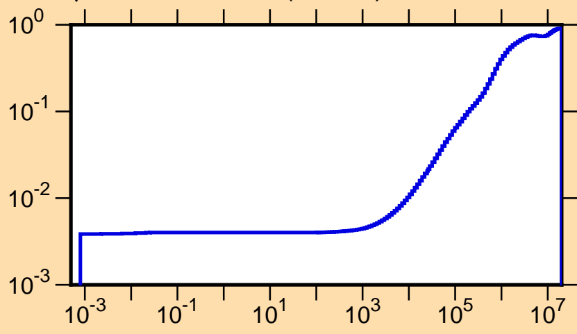
\mu vs. E for ^{175}\text{Ta}(\text{mt251})
